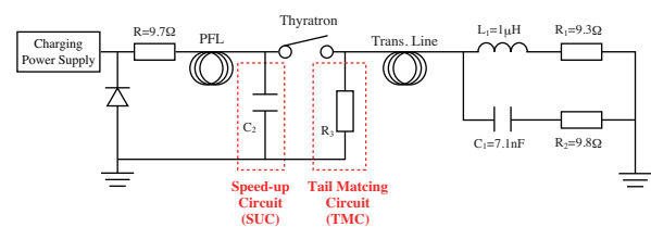
Figure 4: Upgraded circuit.
