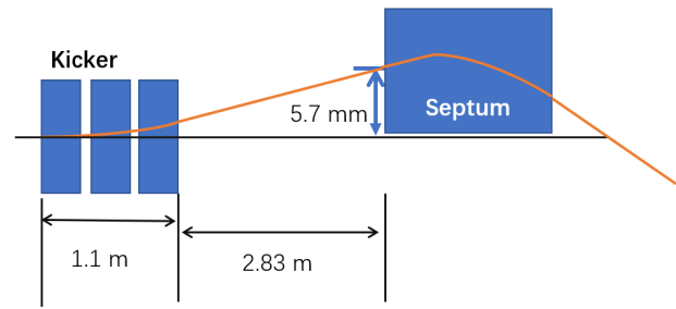
Figure 3: The layout of the vetical injection.
