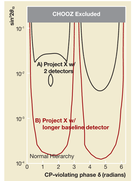
3 \sigma sensitivity to CP-violation assuming the normal mass hierarchy. For the inverted hierarchy, flip each curve around a vertical line through \delta=\pi . All sensitivities assume 3 years of neutrino and 3 years of antineutrino running, corresponding to 60 \times 10^{20} and 120 \times 10^{20} protons on target for each neutrino type for Project X at 120 GeV and 60 GeV, respectively.
