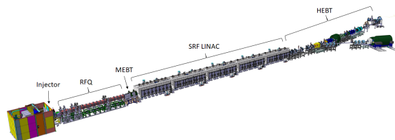
Figure 2: Layout of the IFMIF-DONES AS.
