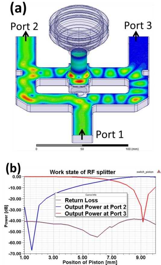
Figure 4: the RF splitter design using WR90 waveguide: (a) geometry; (b) power at each port versus position of the piston.
