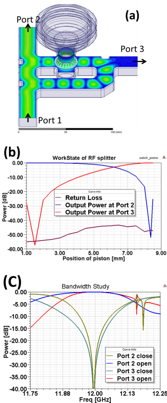
Figure 5: RF splitter design using 20 mm x 12 mm waveguide: (a) geometry; (b) power obtained at each port versus position of piston; (c) bandwidth plots.
