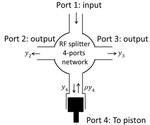
Figure 1: The 4 port network proposal for RF splitter.
