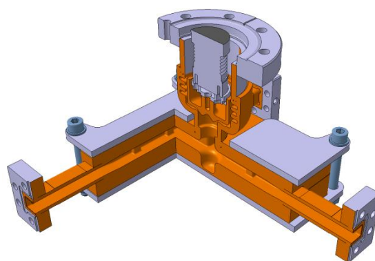
Figure 6: Mechanical design of the variable RF splitter.
