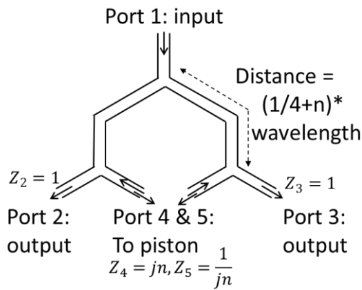
Figure 2: The 5 port network proposal for RF splitter.
