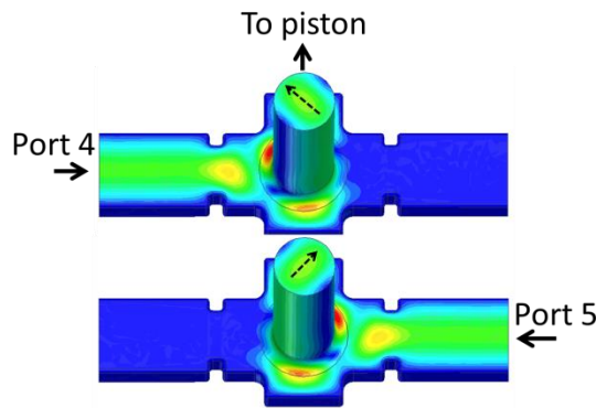
Figure 3: RF polarizer.
