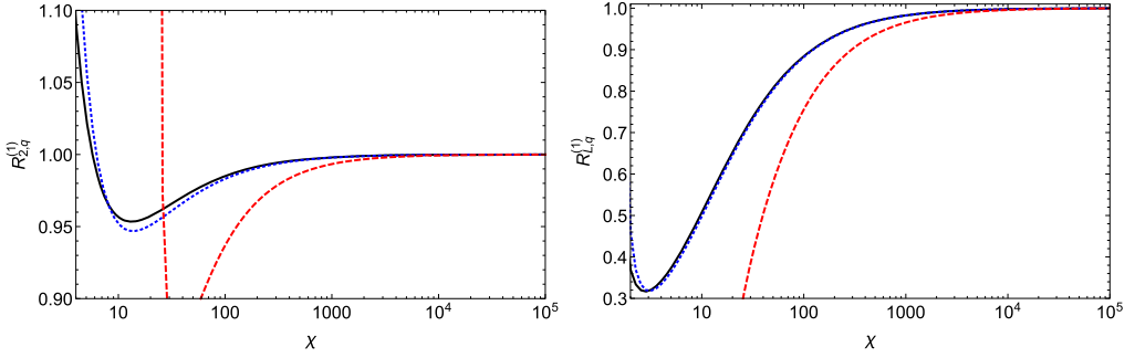
Fig. 3. The ratios R_{2,q}^{(1)} (left) and R_{L,q}^{(1)} (right), Eq. (147), as a function of \chi = Q^2/m^2 . Solid line: z = 10^{-4} ; dotted line: z = 10^{-2} ; dashed line: z = 1/2 .
