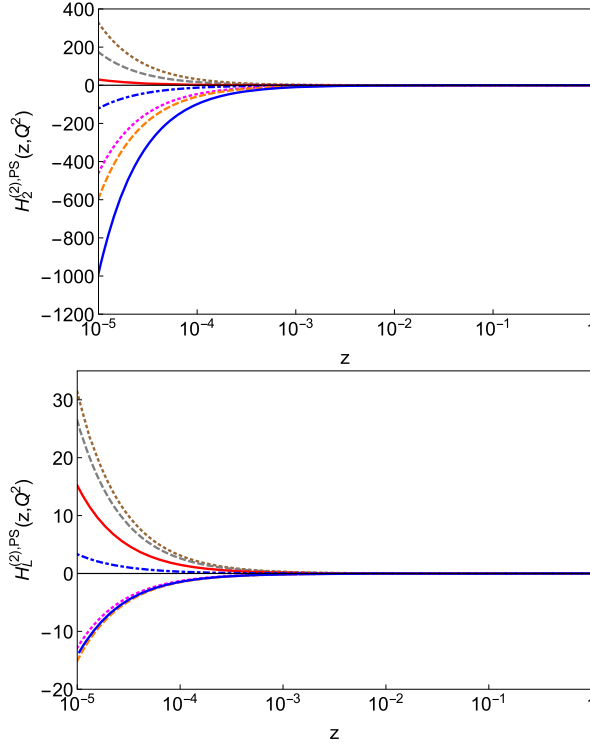
Fig. 2. The Wilson coefficients H_{2,q}^{(2),PS} (upper panel) and H_{L,q}^{(2),PS} (lower panel) as a function of z for different values of Q^2 and the scale choice \mu^2 = \mu_F^2 = Q^2 . Lower full line (Blue): Q^2 = 10^4 GeV 2 ; lower dashed line (Orange): Q^2 = 10^3 GeV 2 ; lower dotted line (Magenta): Q^2 = 500 GeV 2 ; dash-dotted line (Blue): Q^2 = 100 GeV 2 ; upper full line (Red): Q^2 = 50 GeV 2 ; upper dashed line (Gray): Q^2 = 25 GeV 2 ; upper dotted line (Brown): Q^2 = 10 GeV 2 . (For interpretation of the colors in the figure(s), the reader is referred to the web version of this article.)
