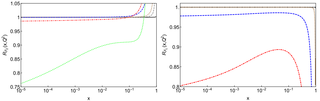
Fig. 7. The ratios of the structure functions F_{2,q}^{2,PS} (left) and F_{L,q}^{2,PS} (right) in the full calculation over the O((m^2/Q^2)^2) improved approximation for different values of Q^2 and the scale choice \mu^2 = \mu_F^2 = Q^2 . Full lines (Black): Q^2 = 10^4 GeV 2 ; dashed lines (Gray): Q^2 = 10^3 GeV 2 ; dotted lines (Brown): Q^2 = 500 GeV 2 ; lower dashed lines (Blue): Q^2 = 100 GeV 2 ; dash-dotted lines (Red): Q^2 = 50 GeV 2 ; lower dotted lines (Green): Q^2 = 25 GeV 2 , using the parameterization of the parton distribution [73].
