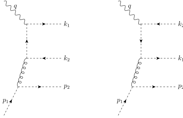
Fig. 8. Diagrams of the O(a_s^2) contributions to the pure singlet scattering cross section \gamma^* + q \rightarrow Q + \bar{Q} + q .
