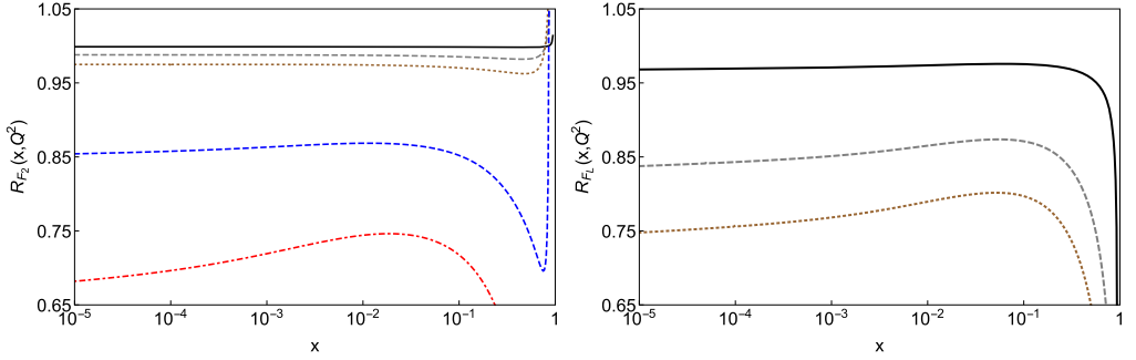
Fig. 6. The ratios of the structure functions F_{2,q}^{(2),PS} (left) and F_{L,q}^{(2),PS} (right) in the full calculation over the asymptotic approximation for different values of Q^2 and the scale choice \mu^2 = \mu_F^2 = Q^2 . Full line (Black): Q^2 = 10^4 GeV 2 ; dashed line (Gray): Q^2 = 10^3 GeV 2 ; dotted line (Brown): Q^2 = 500 GeV 2 ; lower dashed line (Blue): Q^2 = 100 GeV 2 ; dash-dotted line (Red): Q^2 = 50 GeV 2 , using the parameterization of the parton distribution [73].
