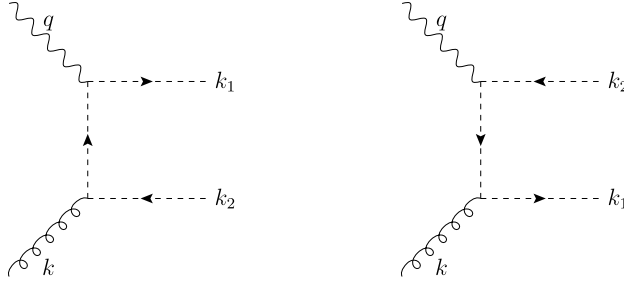
Fig. 1. Diagrams of the O(a_s) contributions to scattering cross section \gamma^* + g \rightarrow q + \bar{q} .
