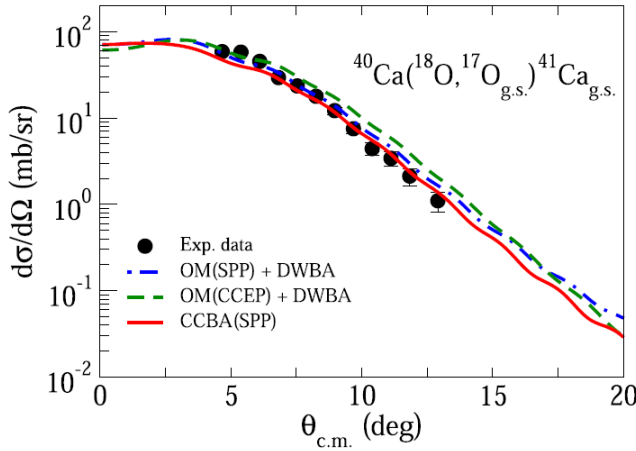
Figure 2. Comparison between theoretical and experimental one-neutron transfer angular distribution for the transition ^{40}\text{Ca}(^{18}\text{O}, ^{17}\text{O}_{\text{g.s.}})^{41}\text{Ca}_{\text{g.s.}} . The OM(SPP)+DWBA, OM(CCEP)+DWBA and CCBA(SPP) calculations are indicated by the dash-dotted blue, dashed green, and solid red lines, respectively. Figure from Ref. [28].
