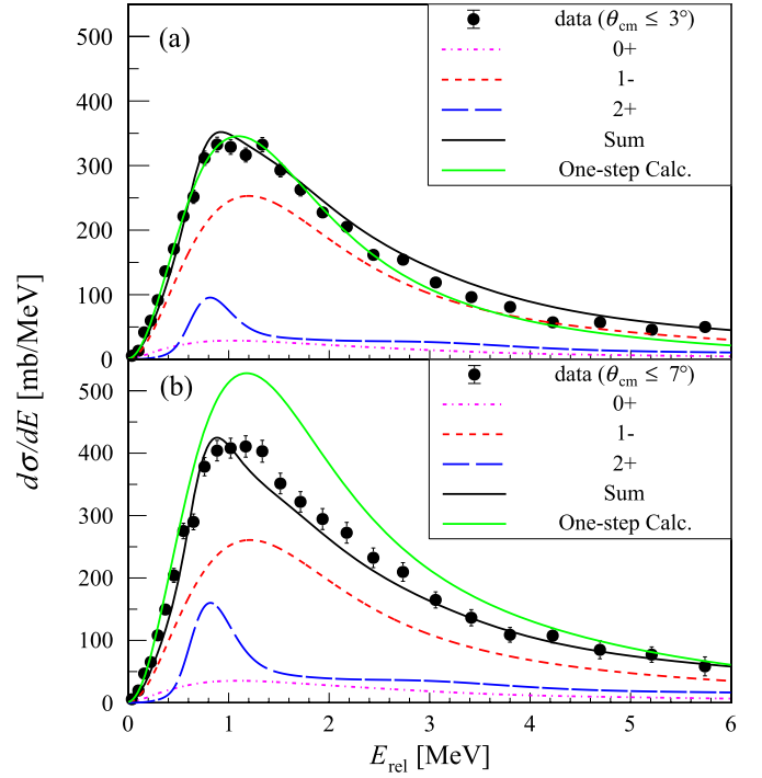
Fig. 2. Breakup cross sections as a function of the three-body relative energy for {}^6\text{He} + \text{Pb} with angular cuts of (a) \theta_{\text{cm}} \leq 3^\circ and (b) \theta_{\text{cm}} \leq 7^\circ . The data is compared with the “modified CDCC” calculations. See text for details.
