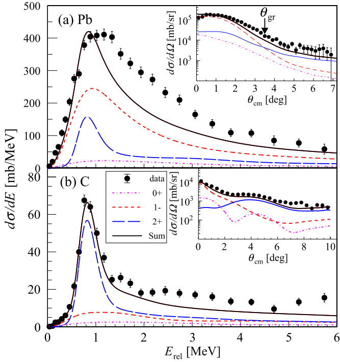
Fig. 1. Breakup cross sections as a function of the three-body relative energy for (a) {}^6\text{He} + \text{Pb} with \theta_{\text{cm}} \leq 7^\circ and (b) {}^6\text{He} + \text{C} with \theta_{\text{cm}} \leq 10^\circ . The insets show the scattering angular distributions in the center-of-mass frame of {}^6\text{He} + \text{target} . \theta_{\text{gr}} denotes the grazing angle of 3.45^\circ . The data is compared with the four-body CDCC calculations (black solid lines) decomposed to 0^+ (magenta dotted-dash lines), 1^- (red dashed lines) and 2^+ (blue dashed lines) continuum states.
