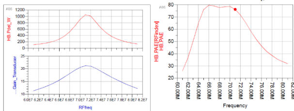
Figure 6: Final results of 1 kW power amplifier design.
