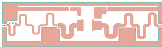
Figure 5: PCB design of 1 kW power amplifier with input transformer.
