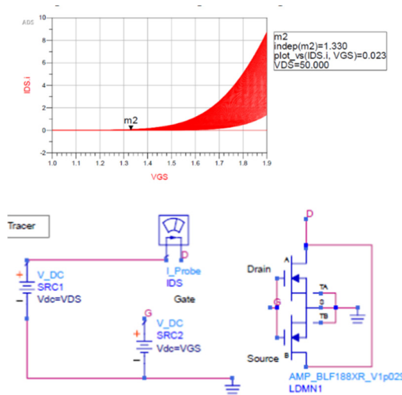
Figure 1: Schematic of DC analysis and diagram of drain current in terms of gate voltage.
