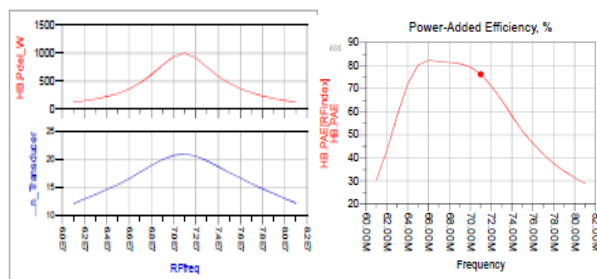
Figure 7: Final results of 1 kW power amplifier design with input transformer.
