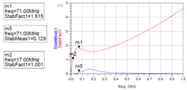
Figure 2: Stability analysis of the transistor.
