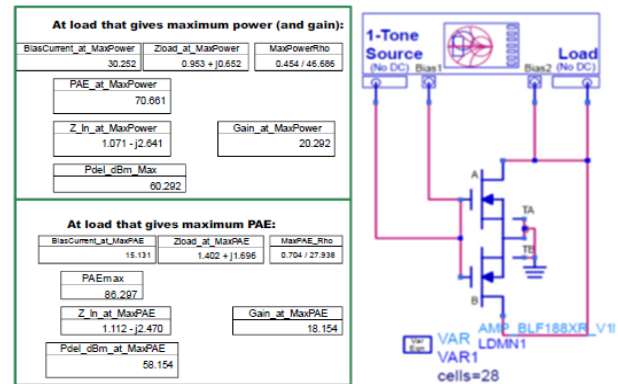
Figure 3: Load-Pull analysis of the transistor.
