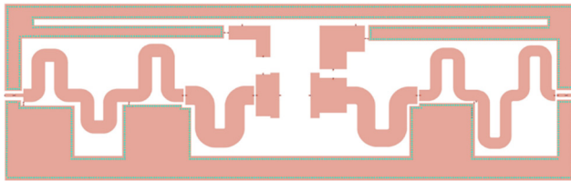
Figure 4: PCB design of the 1 kW power amplifier.
