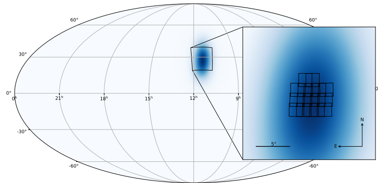
Figure 5. The target of the opportunity observation program produced the observation grids and the observation pointing sequences for GRB 220321A. The trigger number is 669537987, and the probability data from GCN Circular [68].
