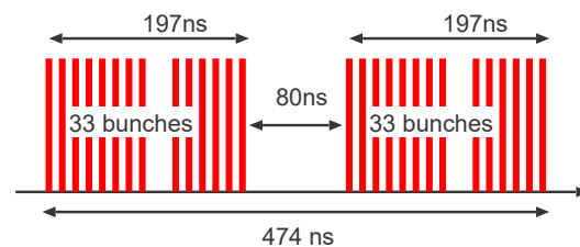
Figure 2: The beam structure in the positron source for the 39 mini-train case. Each mini-train contains 33 bunches. Each pulses contain 2 or 1 mini-trains.
