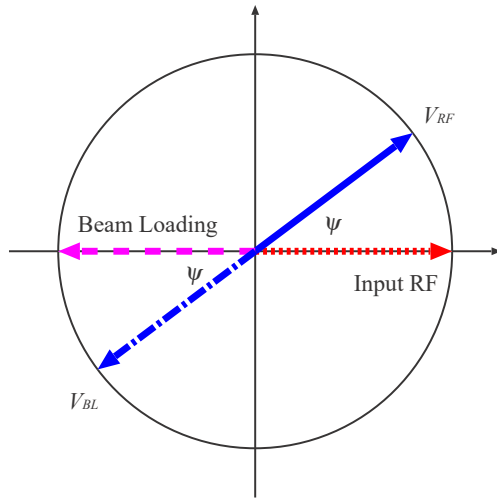
Figure 4: Phase diagram of cavity voltage with a detuning angle. Input RF is defined as zero phase shown with a dashed line arrow. The induced voltage by RF ( V_{RF} ) has an angle \psi from the input RF shown with a solid line. The beam loading input is opposite phase to the input RF. The induced voltage by Beam loading V_{BL} has an angle \psi from the beam loading input.
