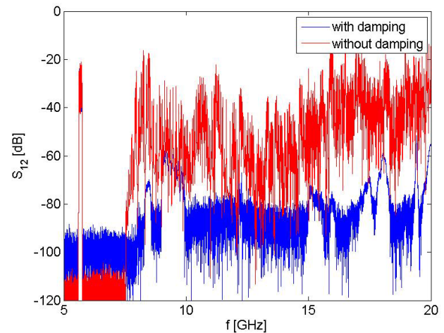
Figure 7: Transmission coeff. between two antennas coupled to a 12 cell module with and w/o the absorbers.
