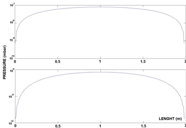
Figure 5: Pressure profile along the axis of the structure for two different values of the specific outgassing rate.
