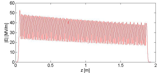
Figure 3: Accelerating field on axis.
