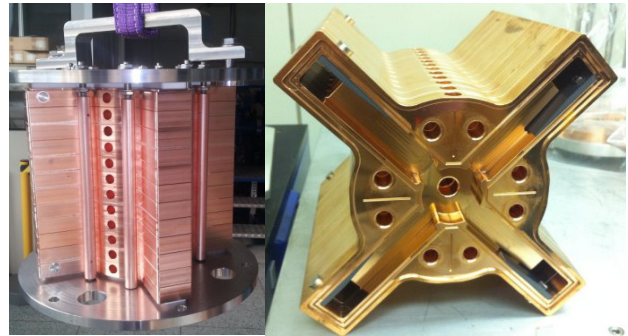
Figure 6: Picture of a single 12 cell module of the “mechanical prototype” after brazing (left) and of the “RF prototype” (right).
