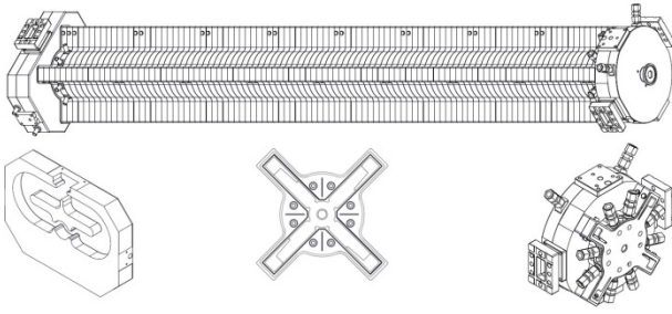
Figure 1: C-Band travelling wave structures.
