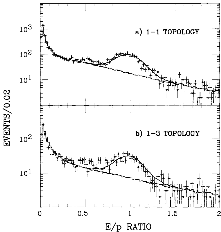
Fig. 1 Energy/momentum ratio for one-prong tau decays compared to the fits described in the text: (a) one-prong tau decays from the 1-1 decay topology, (b) one-prong tau decays from the 1-3 decay topology.
