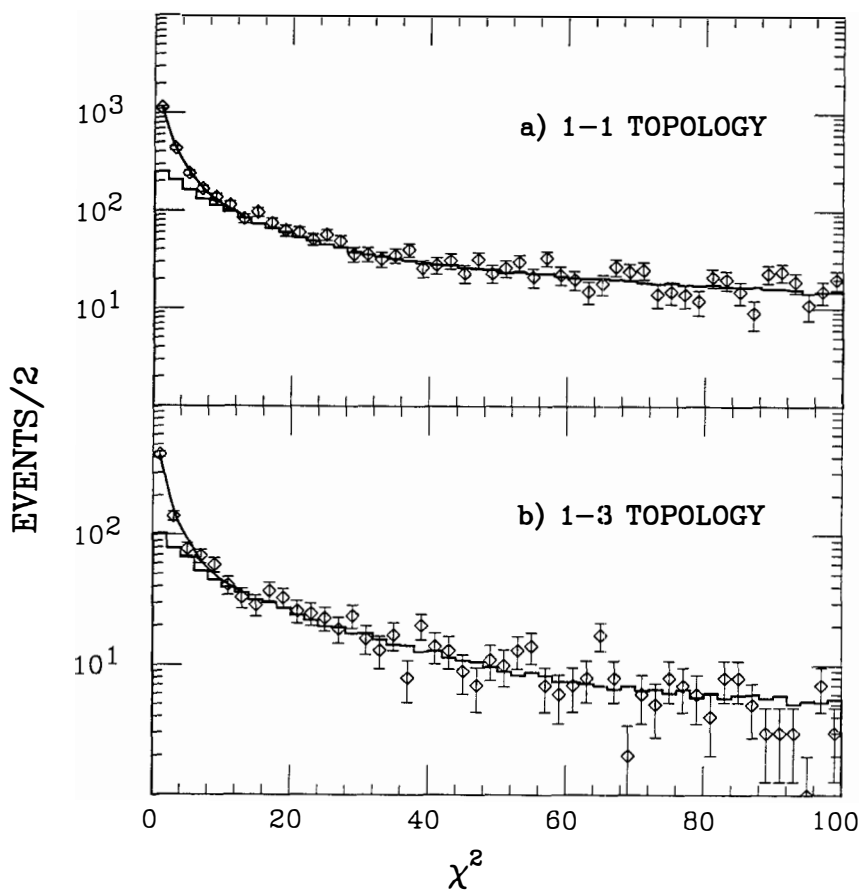
Fig. 2 Distribution in \chi^2 (equation (2)) compared to the fits described in the text: (a) one-prong tau decays from the 1-1 decay topology, (b) one-prong tau decays from 1-3 decay topology.
