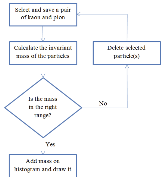
Figure 6: Algorithm for analysing a single event
