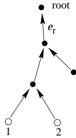
Figure 1. Numbered tree, non-numbered vertices are black.
