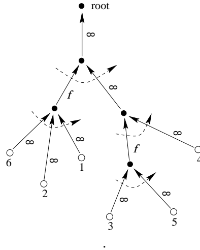
Figure 4. A planar tree which gives a 2-dimensional cell in K_6
