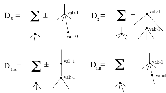
Figure 16. Decomposition of terms of type D.
