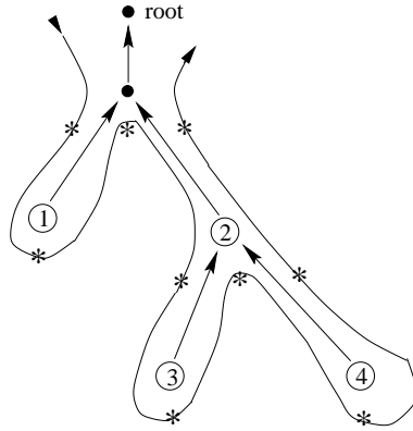
Figure 7. A path from the left to the right passing through all angles.
