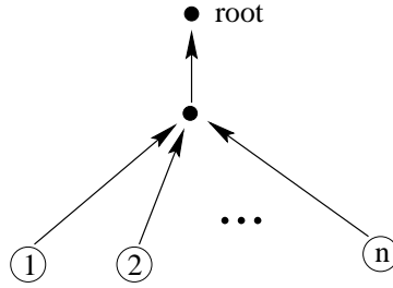
Figure 11. The unique abstract tree which is not killed by the projection from G_n to the space of generators.
