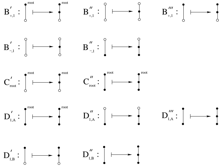
Figure 17. Further decompositions of terms B_{+1}, B_{-1}, D_{1,A}, D_{1,B} .
