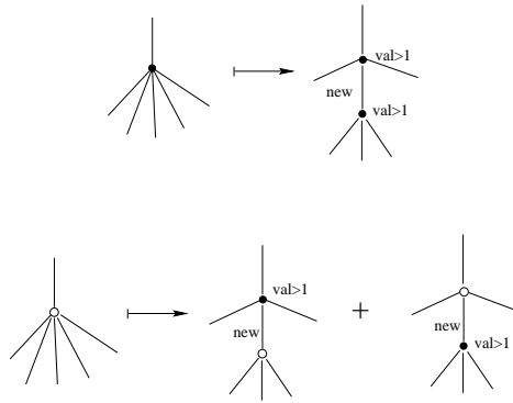
Figure 10. Two types of terms in the formula for differential in M .
