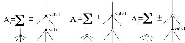
Figure 13. Decomposition of terms of type A.
