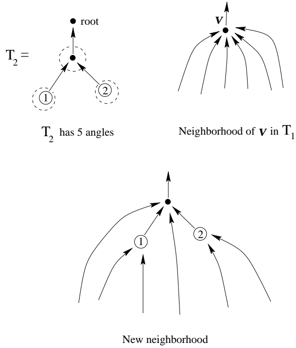
Figure 8. A way to insert tree T_2 in the place of vertex v in tree T_1 .
