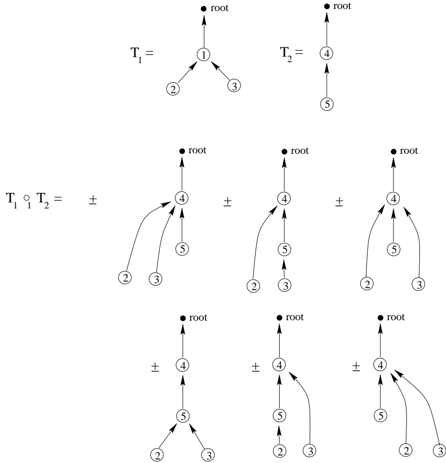
Figure 9. An example of the composition in M .
