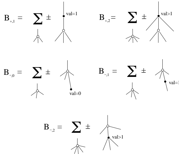
Figure 14. Decomposition of terms of type B.
