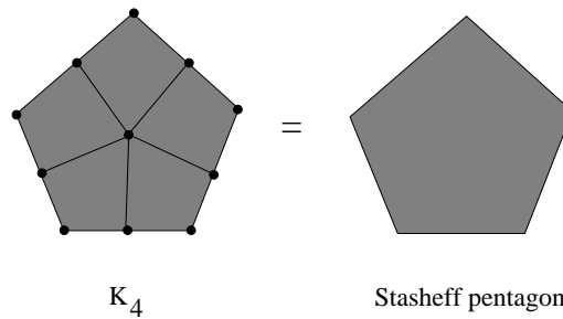
Figure 5. Cell complex K_4 has 11 vertices, 15 edges and 5 two-dimensional faces. It is homeomorphic to the Stasheff pentagon.
