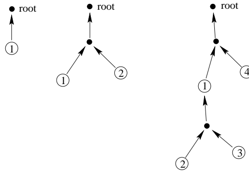
Figure 6. Three examples of admissible labeled planar trees.
