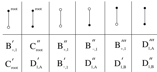
Figure 17. Further decompositions of terms B_{+1}, B_{-1}, D_{1,A}, D_{1,B} .
