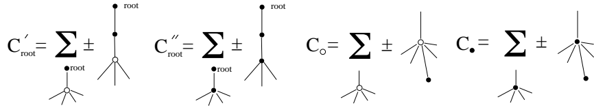
Figure 15. Decomposition of terms of type C.
