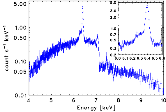
Figure 2: GX 301-2 X-ray spectrum obtained with Chandra HETGS. Blown-up of the iron K\alpha spectrum is also shown. A Compton shoulder is clearly seen in the low energy side of the iron K\alpha line.
