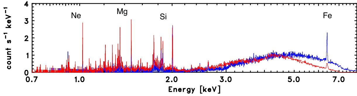
Figure 1: Vela X-1 X-ray spectrum during orbital phase 0.50 obtained with Chandra HETGS. The red line shows the spectrum with Medium Energy Grating (MEG), and, the blue one shows the spectrum with High Energy Grating (HEG). Many emission lines result from a photoionized plasma.
