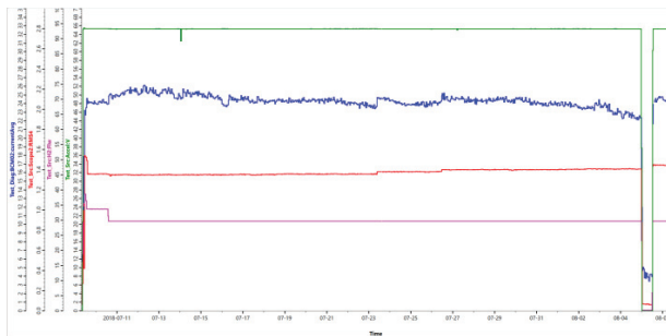
Figure 5: The ion source high voltage (green top trace), the H - beam current (blue 2 nd from top trace), the RF power (red 3 rd from top), and the H 2 flow (pink bottom trace) during the 29 day long run of the SNS source with a 10% duty factor.
