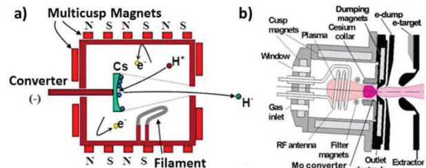
Figure 1: Schematics of a) the LANSCE filament-driven converter- and b) the SNS RF driven- H^- ion sources.
