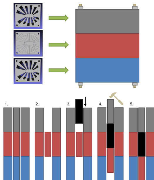
Figure 5: Assembly tooling and magnet insertion process.
