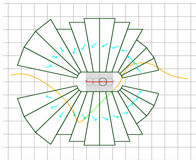
Figure 1: 2D permanent magnet design (cm grid). Midplane field is graphed in orange, with good field region in green.
