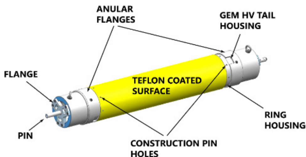
Figure 9. Drawing of the mold used for the sub-layer. Arrows indicate some details that are useful during the construction. Reprinted with permission from Reference [26].
