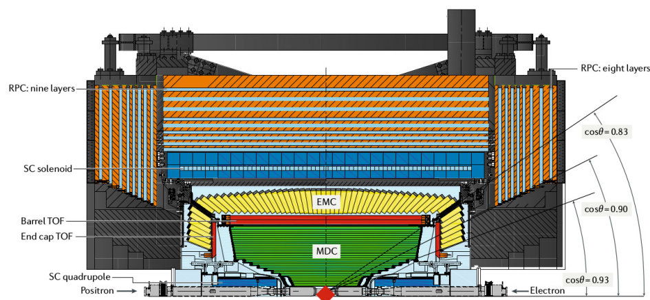
Figure 1. BESIII spectrometer layout: the beam pipe is at the bottom of the picture where the red diamond identifies the interaction point. Each detection system is highlighted in a different color. The full detector has a cylindrical symmetry around the beam pipe, a radius of 2.5 m, and a length of 5.6 m.
