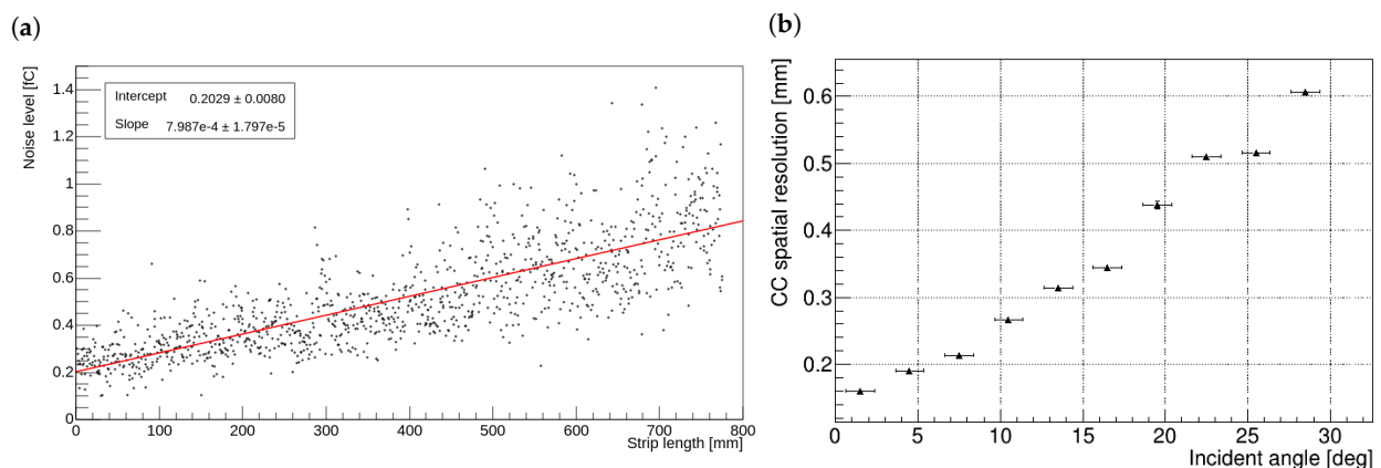
Figure 33. Preliminary results from the CGEM-IT cosmic setup with two final layers at IHEP. (a) Measured noise as a function of the V strip length for the CGEM-IT inner layer; longer strips have a larger capacitance and thus a higher noise [21]. (b) CC resolution of the CGEM-IT inner layer as a function of the track incident angle; the tracking system contribution is not subtracted [90].
