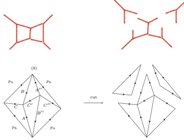
Figure 7.13: Example of a cut contributing to the final result.
