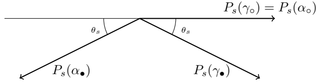
Figure 5.3: Projections of the root \gamma_\circ = \alpha_\circ , \gamma_\bullet = w^{-1}\alpha_\bullet and \alpha_\bullet on the eigenplane of w spanned by z_s and z_{h-s} . By \circ and \bullet we respectively mean any element in \circ and \bullet and we defined \theta_s \equiv \frac{\pi s}{h} .
