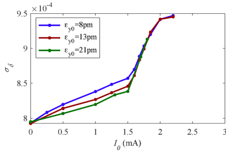
Figure 7: The energy spread vs. single bunch current numerically simulated by the ELEGANT code with IBS and the total longitudinal wakefield.
