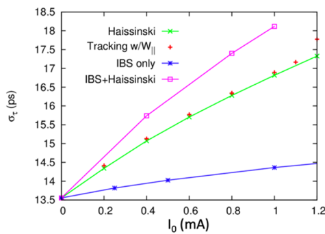
Figure 4: The bunch length as a function of single bunch current. The blue trace includes IBS only. The green trace represents the results of the numerical simulations using a Haissinski solver. The red crosses are tracking with the total longitudinal wakefield. The magenta trace is the combined effect of IBS and the Haissinski solution.
