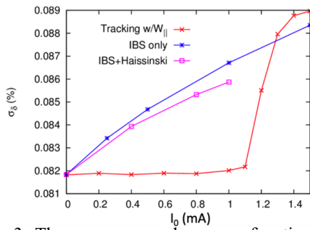
Figure 3: The energy spread \sigma_\delta as a function of single-bunch current I_0 obtained by particle tracking simulations. The red trace includes the total wakefield only. The blue trace is the result estimated with the IBS effect only. Magenta trace includes IBS and bunch lengthening effect (Haissinski solution).
