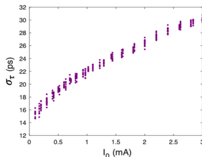
Figure 2: The measured bunch length as a function of single bunch current for the 3DW regular lattice at V_{RF} = 3 MV.
