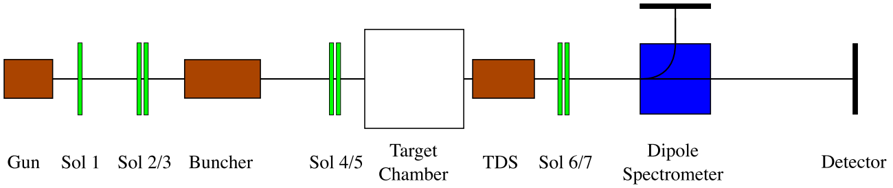
Figure 1: Schematic overview of the REGAE beamline featuring the rf cavities (brown), magnetic solenoids (green), dipole spectrometer (blue) and detector screens (black). The position of the target chamber is also indicated.
