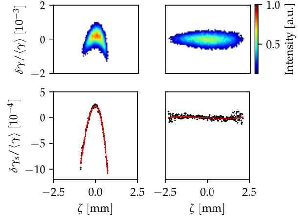
Figure 4: Comparison between on-crest (left) and ESC (right) operation mode; adapted from [8].
