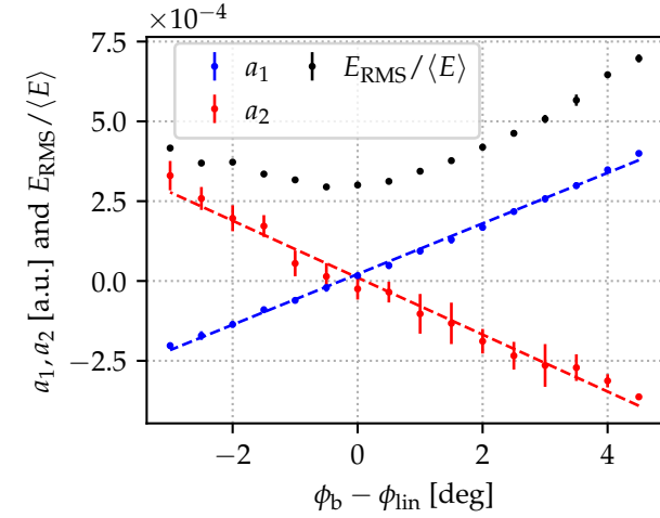
Figure 3: Measurement data of the ESC scheme; adapted from [8].
