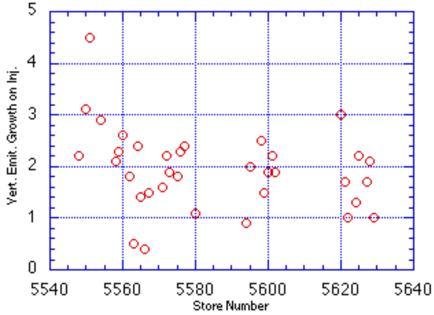
Figure 5 Antiproton Vertical. Emittance Growth on MR to TEV transfer
