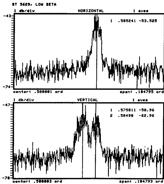
Figure 32. Schottky Signals at Low Beta.
