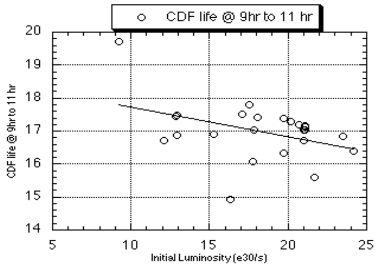
Figure 27 Measured CDF luminosity lifetime at ten hours into the store
