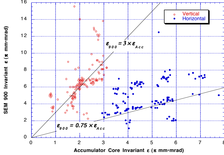
Figure 11. Measured emittances at SEM 900 at the upstream end of the AP3 beamline versus Accumulator core emittances. SEM 900 vertical emittance is plotted against Accumulator vertical emittance and SEM 900 horizontal emittance is plotted against Accumulator horizontal emittance. The data shown here was taken during the period from 17 April 1995 to 23 July 1995. Each point represents a single antiproton transfer.
