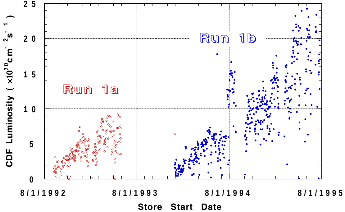
Figure 1. Initial luminosity as reported by CDF for all the stores of Run 1.
