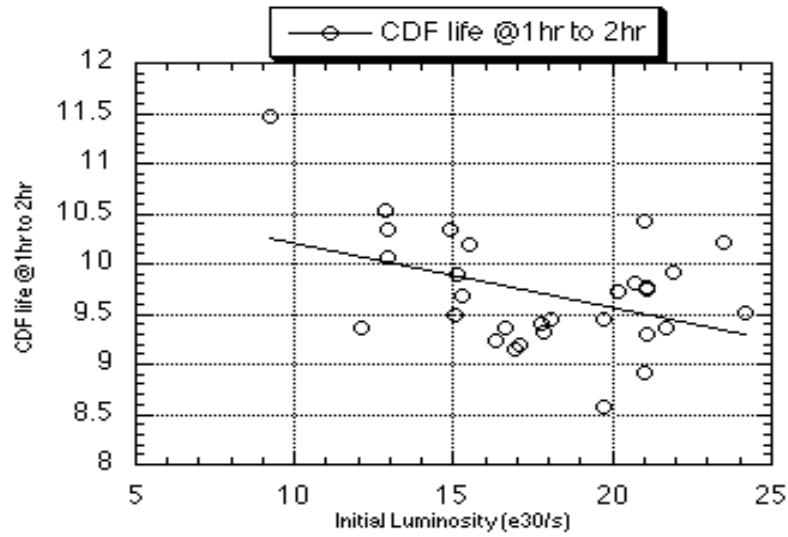
Figure 26 Measured CDF luminosity lifetime in the second hour of the store
