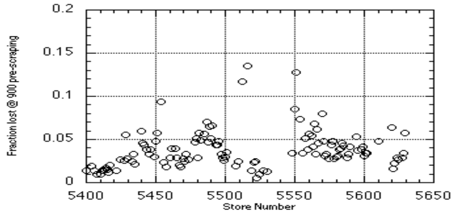
Figure 15 Antiproton Losses at 900 GeV Before Scraping in Tevatron
