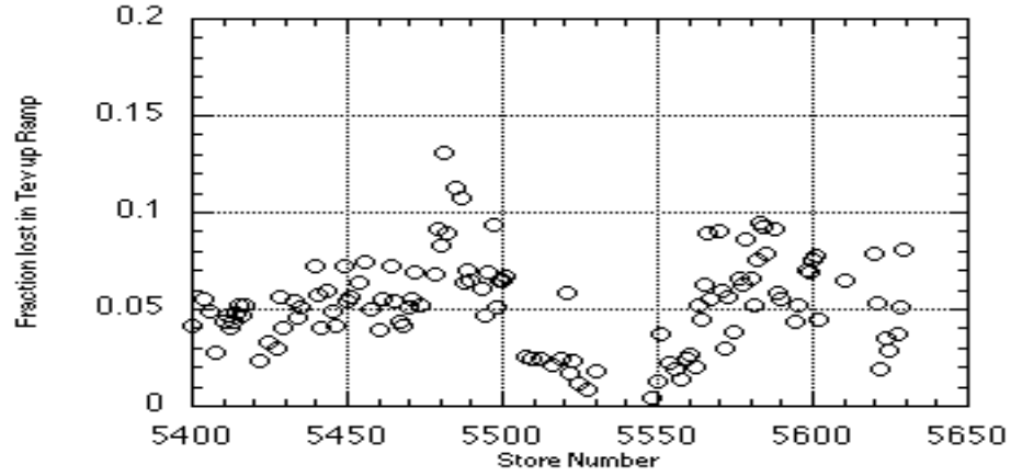
Figure 14 Antiproton Losses up the Ramp in Tevatron
