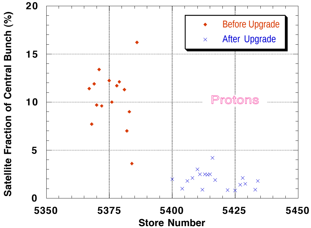
Fig. 3 Proton Satellite percentage before and after the coalescing upgrade.
