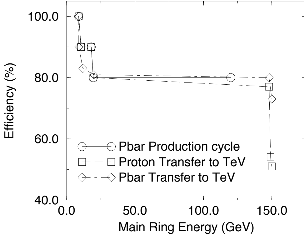
Fig. 1 Main Ring Transfer efficiencies for different particle transfer cycles.
