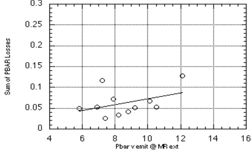
Figure 17 Sum of \bar{p} Losses during the record running period as a function of MR extraction vertical emittance (Runs 5500-5550)
