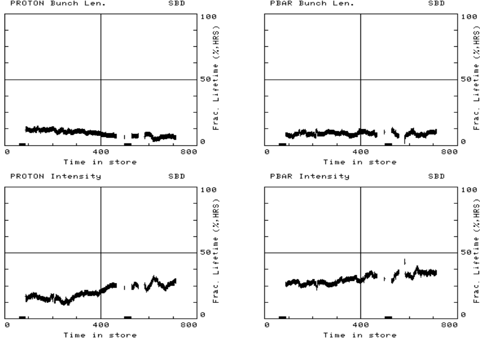
Figure 23 Bunch Length & Intensities Contribution to Luminosity Lifetime for Store 5416
