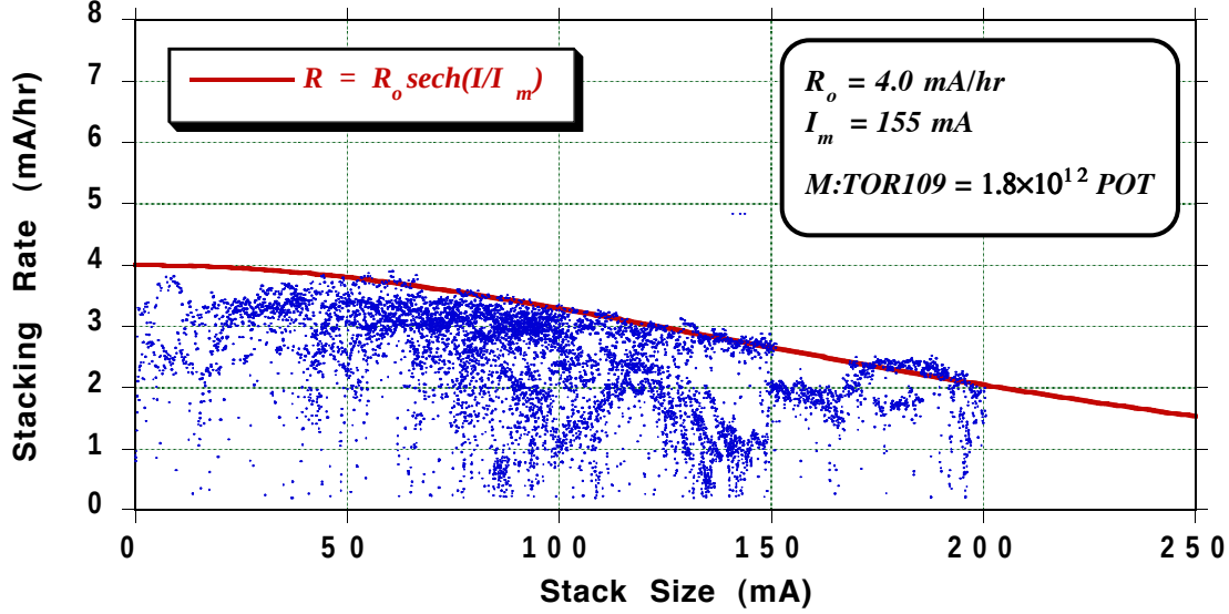
Figure 2. Stacking rate versus stack size for the month of December 1993.
