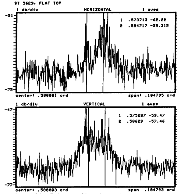
Figure 31. Schottky Signals at Flat Top.
