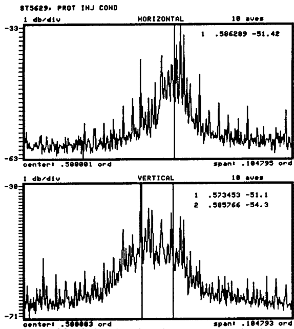
Figure 28. Schottky signals at Proton Injection.
