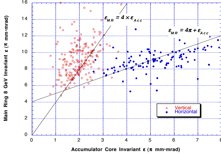
Figure 10. Main Ring flying wire emittances at 8 GeV versus Accumulator core emittances. Main Ring vertical emittance is plotted against Accumulator vertical emittance and Main Ring horizontal emittance is plotted against Accumulator horizontal emittance. The Accumulator emittances are measured using transverse Schottky pickups. Each point in these plots represents the average of all antiproton transfers during the course of a shot (usually 6 transfers). The solid lines indicate that the vertical emittance blows up by at least a factor of 4 while the horizontal emittance growth is 4\pi mm•mrad independent of initial emittance. Some of this 4\pi offset may be measurement error.
