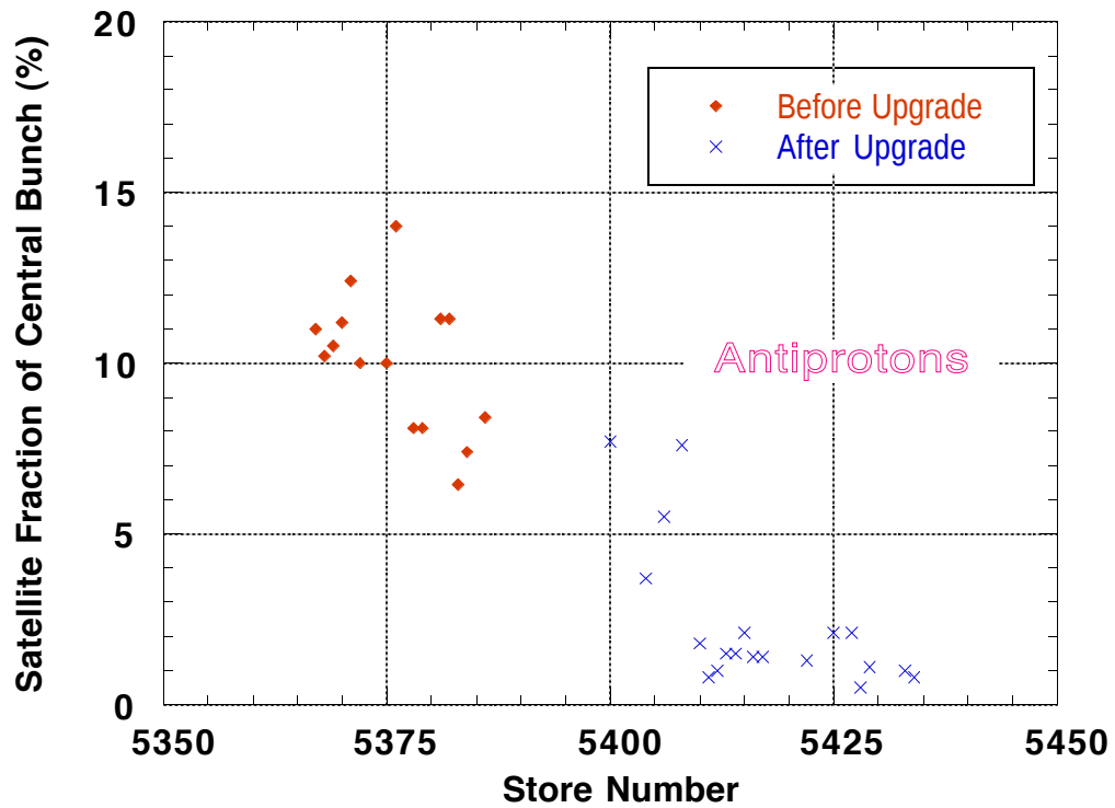
Fig. 5 Antiproton Satellite percentage before and after the Coalescing Upgrade
