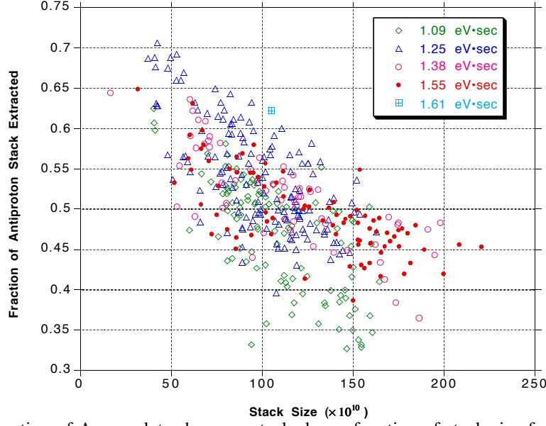
Figure 9. Fraction of Accumulator beam unstacked as a function of stack size for different RF buckets. Note the suppressed zero on the vertical axis.
