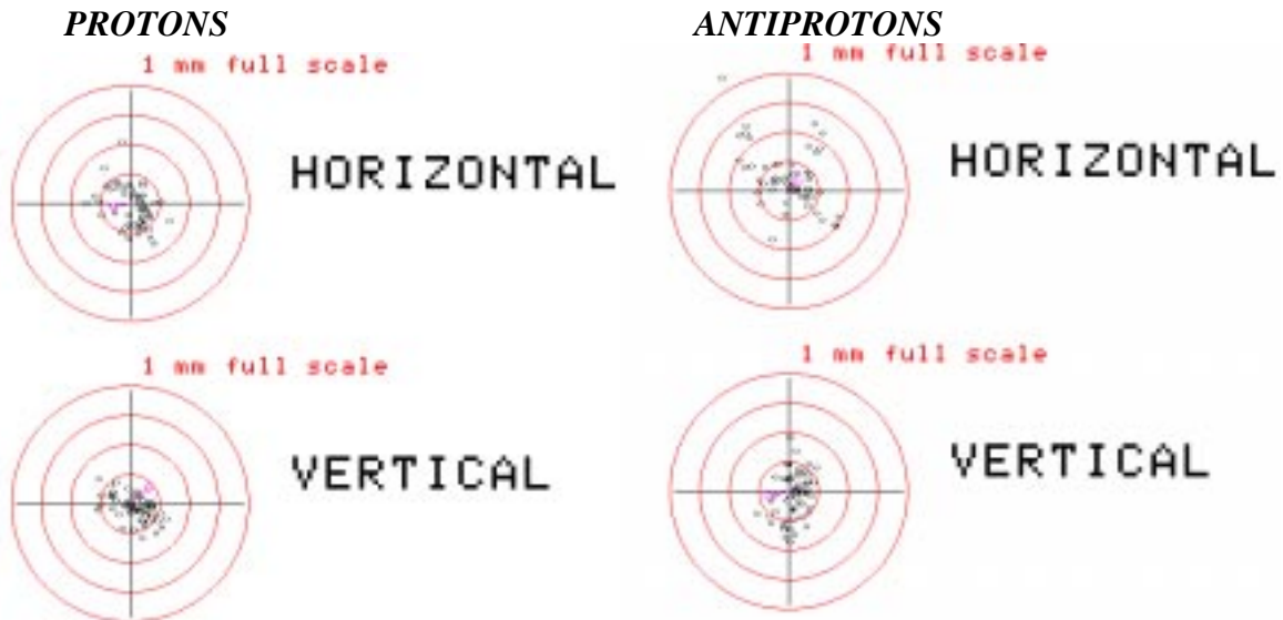
Figure 3 Injection Steering Error Magnitude & Phase for the Most Recent 10 shots (5603-5629)
