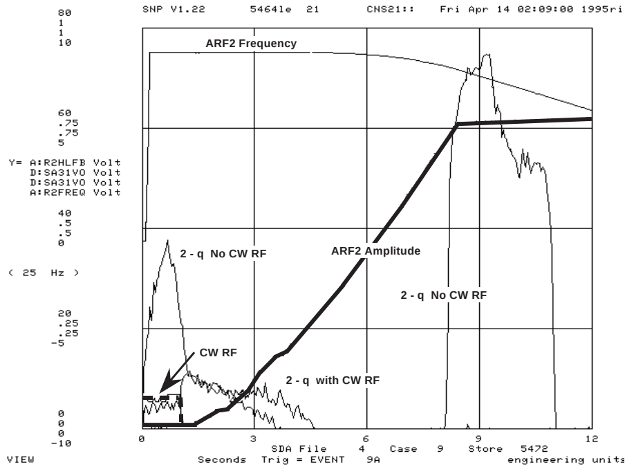
Figure 13. This is a snapshot of several Accumulator parameters during the course of unstacking one antiproton bunch during a collider fill. What is shown here are the first 12 sec of the unstacking sequence (the entire sequence takes 36 sec). Two sequences are superimposed on this plot; one with and one without the CW ion clearing RF. The top curve shows the RF frequency ramp (indicating the revolution frequency of the beam being unstacked). The heavy curve shows the measured voltage on the ARF2 cavity. The heavy dotted curve shows the ARF2 voltage readback with the CW ion clearing RF on. The CW RF is turned off at 1 sec and back on again at 7 sec. The remaining curve on the plot is the amplitude of the beam coherent transverse oscillation at one of its resonant frequencies (the 2 - q resonance). Without the CW RF, there is an initial episode of oscillation for the first second of the cycle - provoked by switching ARF2 from an ion clearing mode to an unstacking mode. There is a second burst of very large amplitude oscillation when the unstacked beam has moved approximately the width of the RF bucket away from the core. When the CW RF is applied the initial oscillation is greatly attenuated and the second period of oscillation is completely absent.
