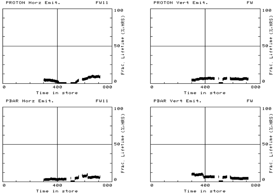
Figure 21 Transverse Growth Contribution to Luminosity Lifetime for Store 5416
