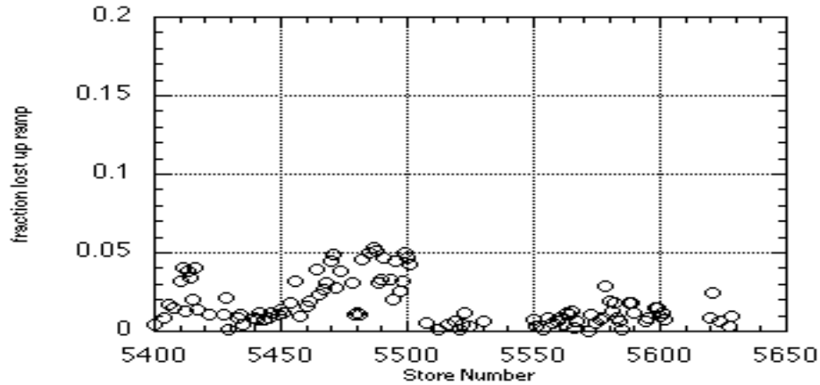
Figure 12 Proton Losses up the Ramp in Tevatron
