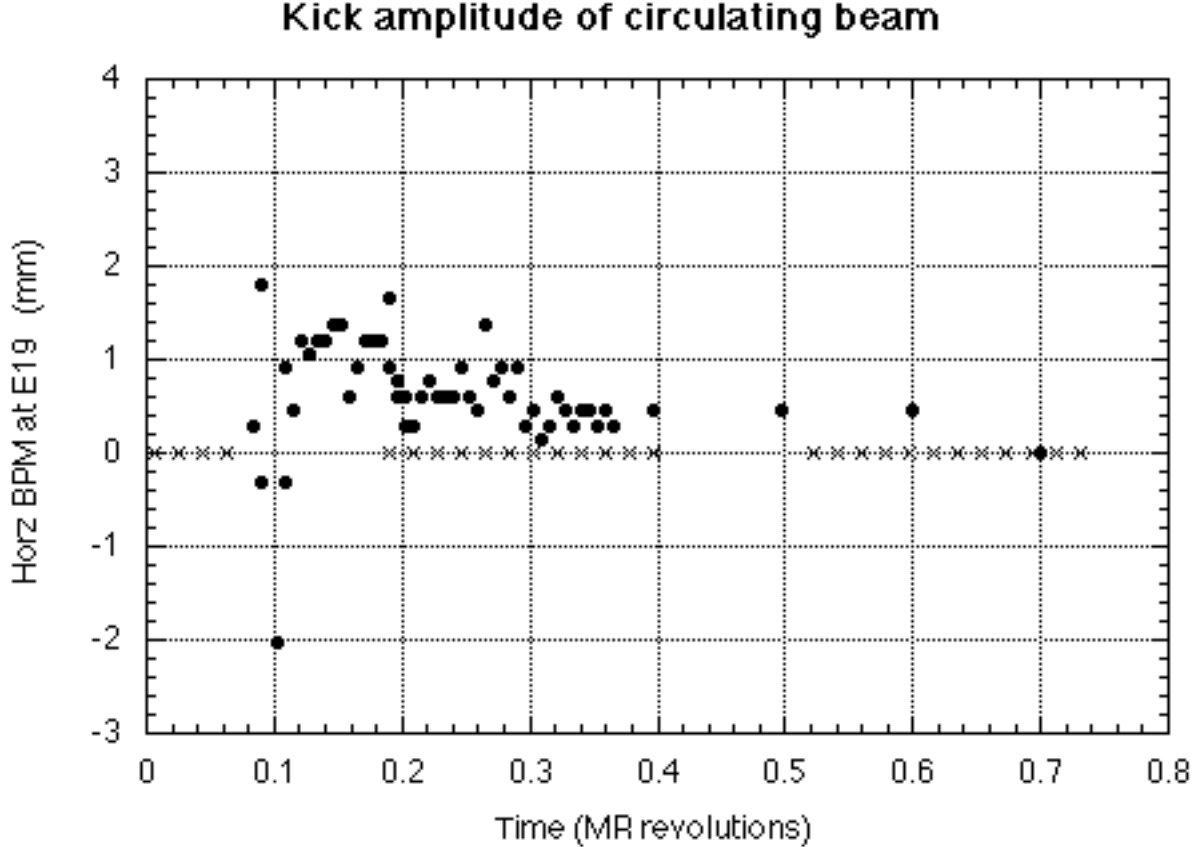
Figure 8 Observed Beam Motion as a Function of Time after Injection Kicker Firing
