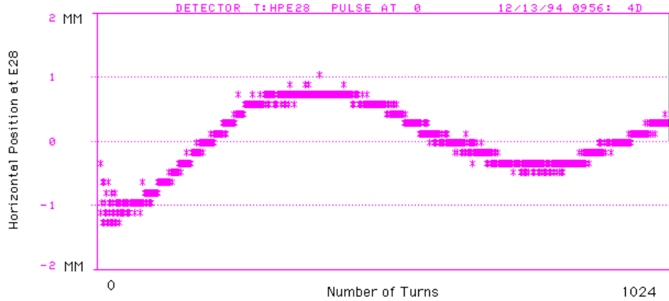
Figure 2 Horizontal TBT for P1 shot 5272
