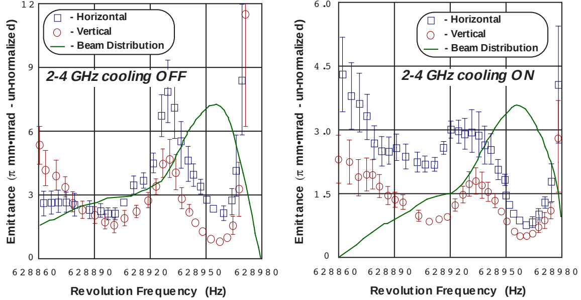
Figure 5. Effect of the 2-4 GHz transverse core cooling system on overcoming the emittance growth due to heating from the stacktail momentum cooling at a revolution frequency of 628930 Hz. The stack size in each case was 135 mA. Note that the vertical scale on the right hand plot is expanded by a factor of two relative to the left-hand plot.
