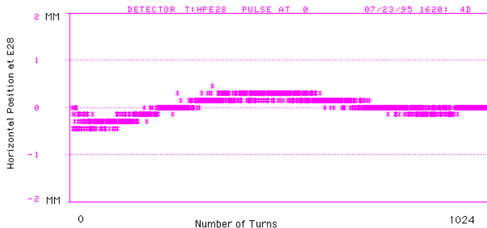
Figure 1 Horizontal TBT for P1 shot 5629
