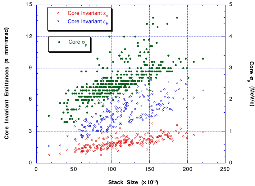
Figure 8. Accumulator core beam size prior to unstacking. In general, the beam is cooled in each dimension to the smallest size possible prior to initiating antiproton transfers.
