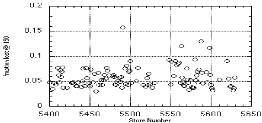
Figure 10 Proton Losses at 150 GeV in Tevatron
