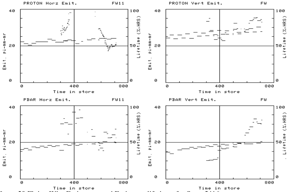
Figure 20 Flying Wire Emittances and Emittance lifetimes for Store 5416
