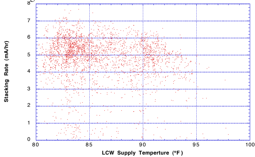
Figure 6. Antiproton stacking rate versus LCW supply temperature for the period from 1 March 1995 through 24 July 1995.
