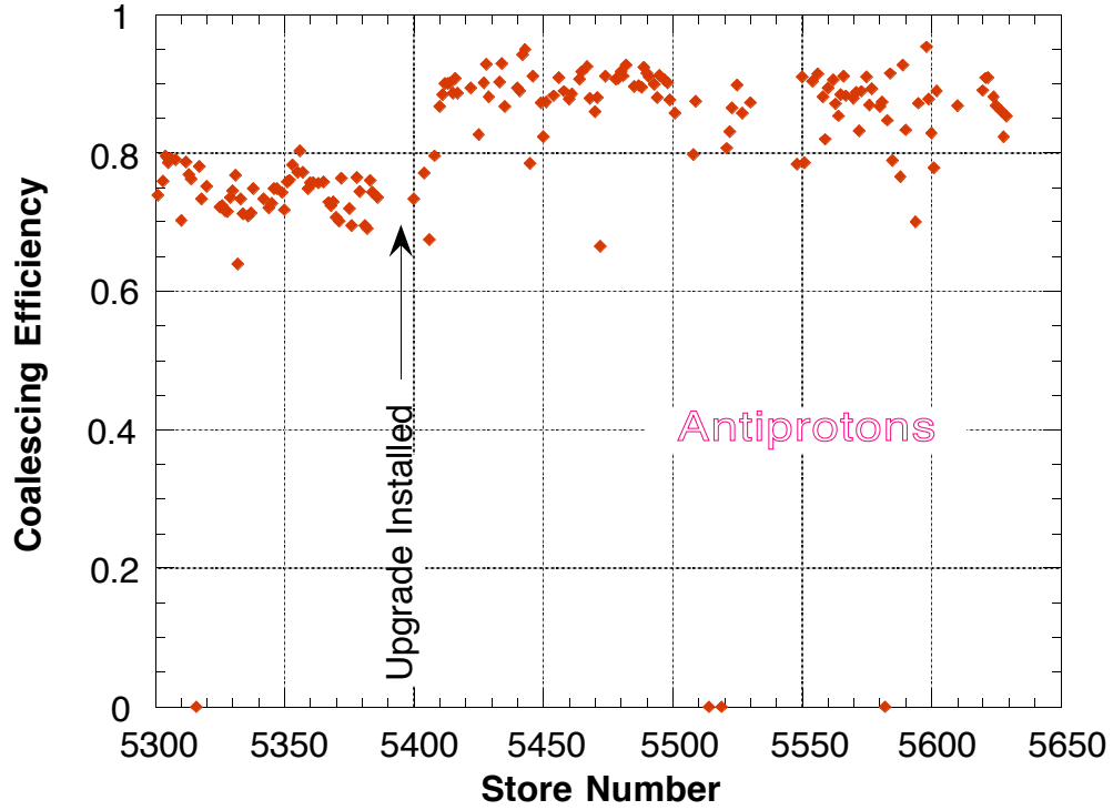
Fig. 4 The antiproton coalescing efficiency before and after the coalescing upgrade
