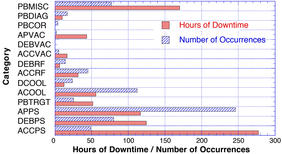
Figure 15. Summary of the antiproton source downtime for Run 1b.
