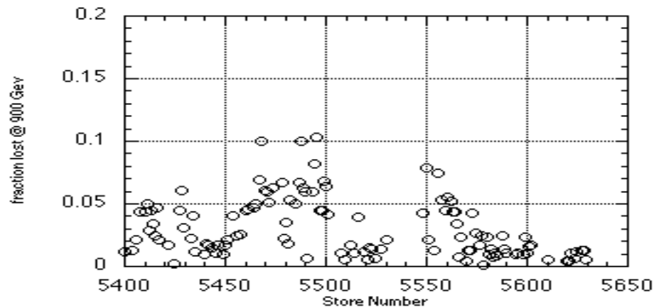
Figure 13 Proton Losses at 900 GeV Before Scraping in Tevatron
