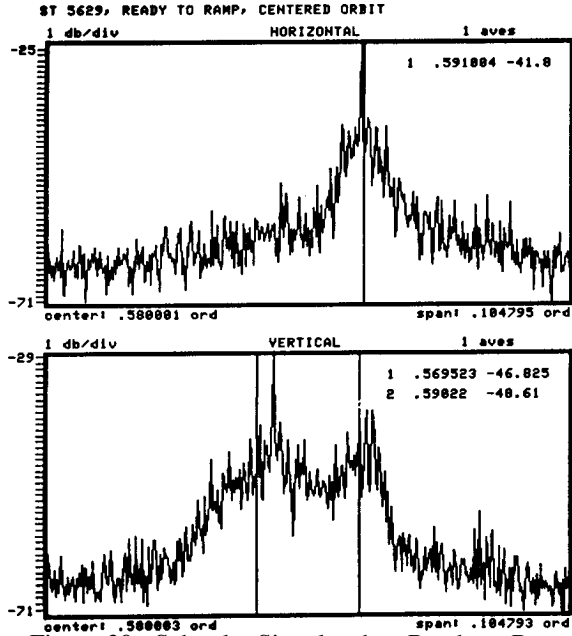
Figure 30. Schottky Signals when Ready to Ramp.
