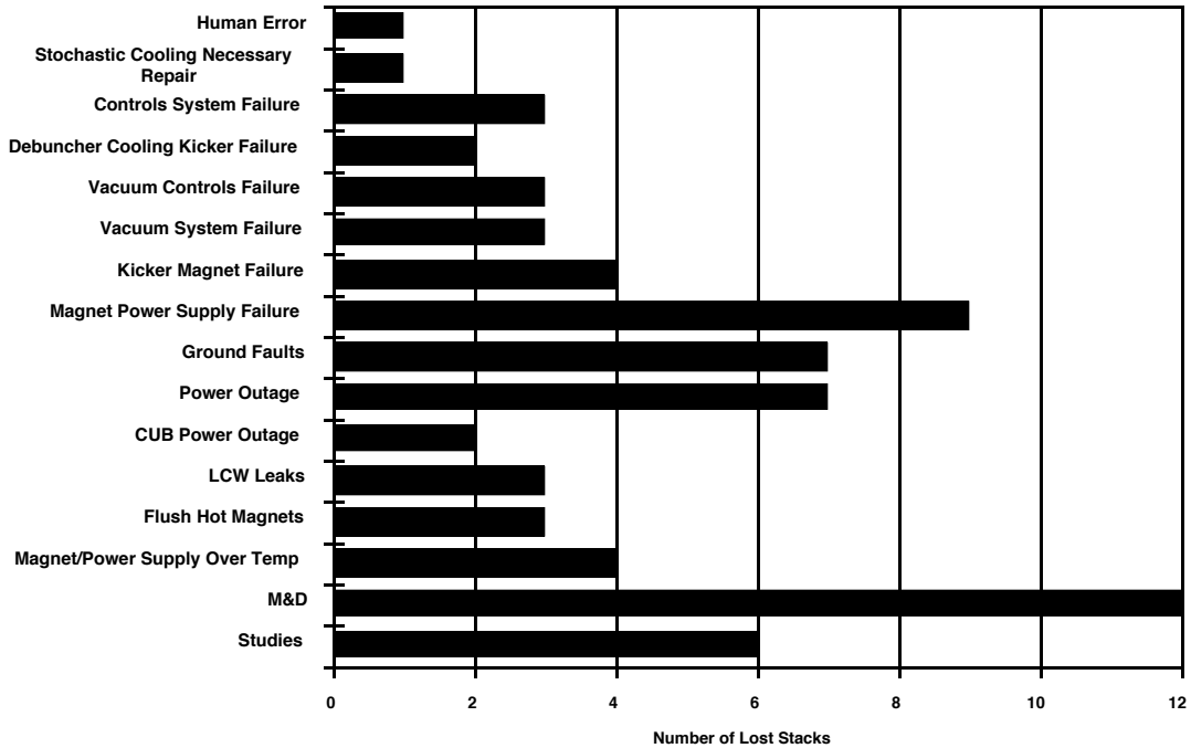
Figure 14. Causes of lost antiproton stacks.
