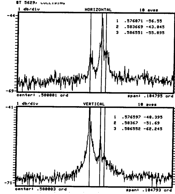
Figure 33. Schottky Signals at Collisions.
