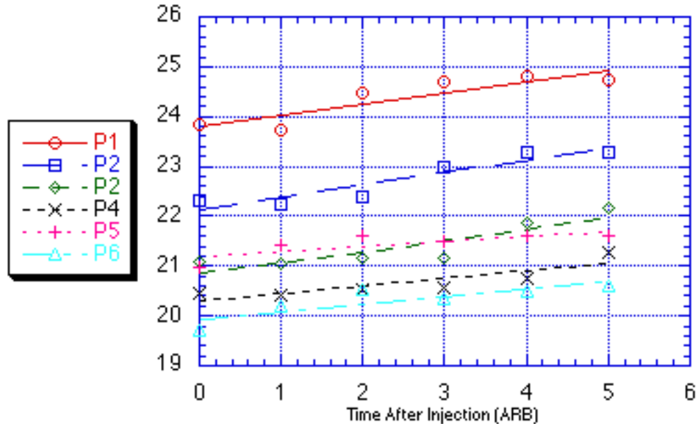
Figure 7 Proton Vertical. Emittance When Later antiproton Bunches are Injected
