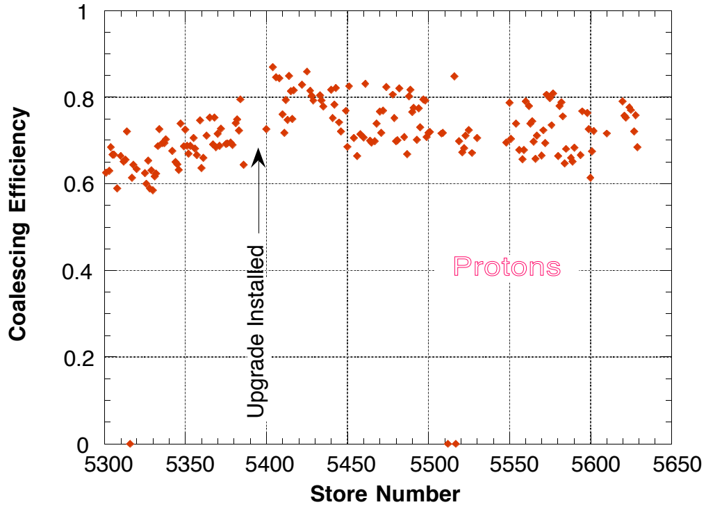
Fig. 2 The Proton Coalescing efficiency before and after the coalescing upgrade
