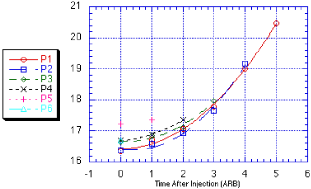
Figure 6 Proton Vertical. Emittance When Later Proton Bunches are Injected
