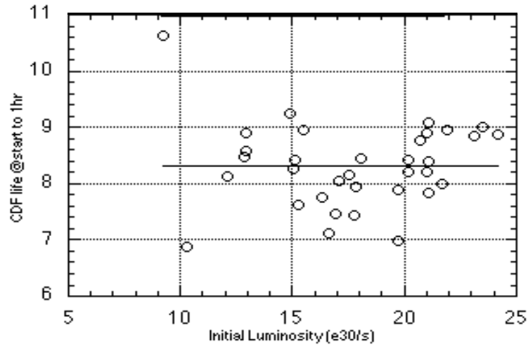
Figure 25 Measured CDF luminosity lifetime in the first hour of the store
