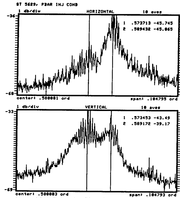
Figure 29. Schottky Signals at \bar{p} Injection.
