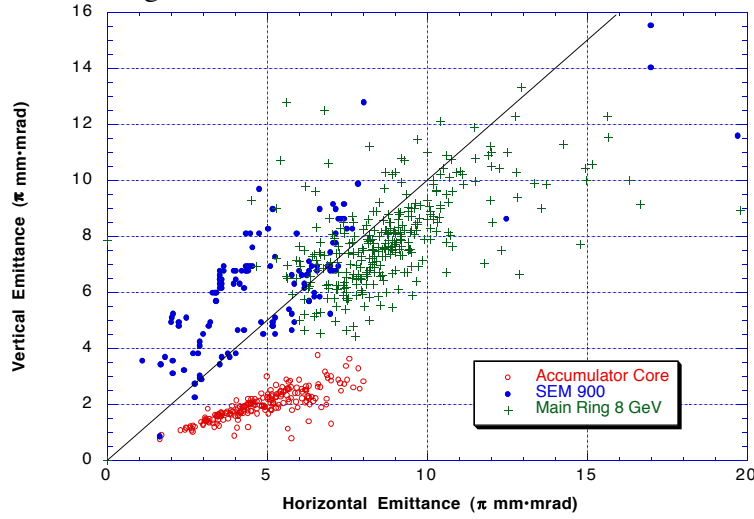
Figure 12. Vertical emittance versus horizontal emittance at the Accumulator core, SEM 900, and Main Ring at 8 GeV. The core and Main Ring data are averages over all transfers in a shot and represent all of Run 1b (i.e. the same data displayed in Figure 10). The SEM 900 data represent individual antiproton transfers during the period 17 April to 23 July 1995 (i.e. the same data displayed in Figure 11).
