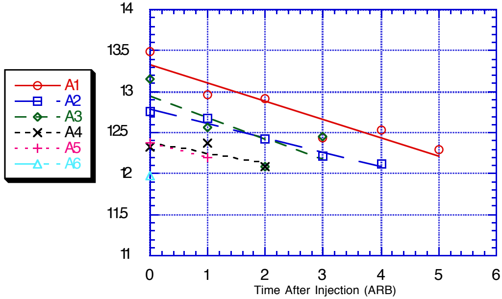
Figure 9 \bar{p} Vertical Emittance as Function of Time after \bar{p} Injection
