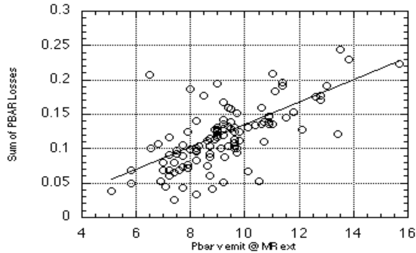
Figure 16 Sum of Antiproton Losses as a Function of MR Extraction Vertical Emittance (Runs 5400-5529)
