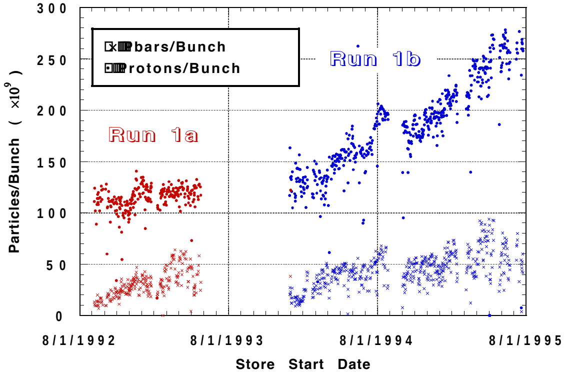
Figure 2. Proton and Antiproton bunch intensities for all the stores of Run 1.
