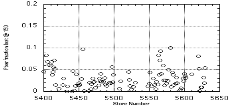
Figure 11 Antiproton Losses at 150 GeV in Tevatron
