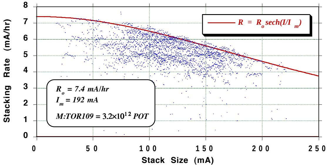
Figure 1. Stacking rate versus stack size for the month of April 1995. One point is plotted for every super cycle during stacking. This month contained the best stacking of Run 1b. POT = Number of protons on target per pulse.
