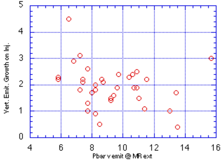
Figure 4 Antiproton Vertical. Emittance Growth on MR to TEV Transfer
