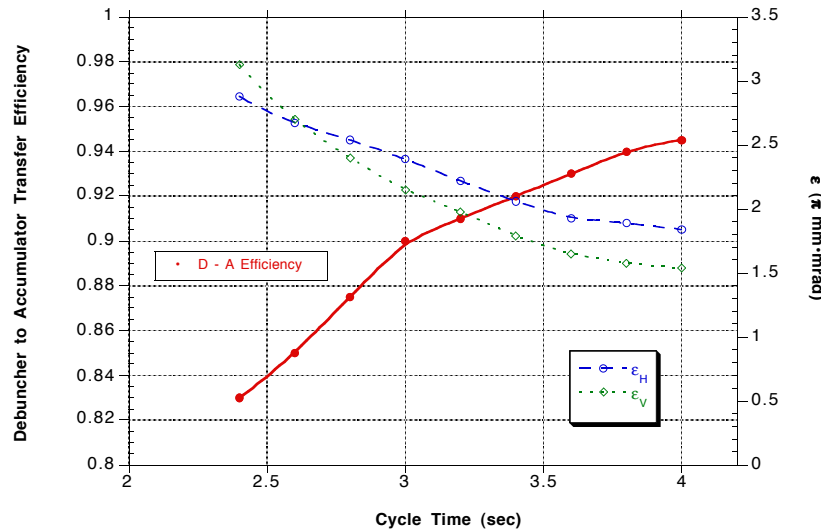
Figure 3. Debuncher to Accumulator transfer efficiency and Debuncher emittances as a function of stacking cycle time. The emittances are measured using a SEM grid in the D-A transfer line (SEM 806). The emittance values plotted in this figure are not normalized. This figure is derived from data taken from reference [3].
