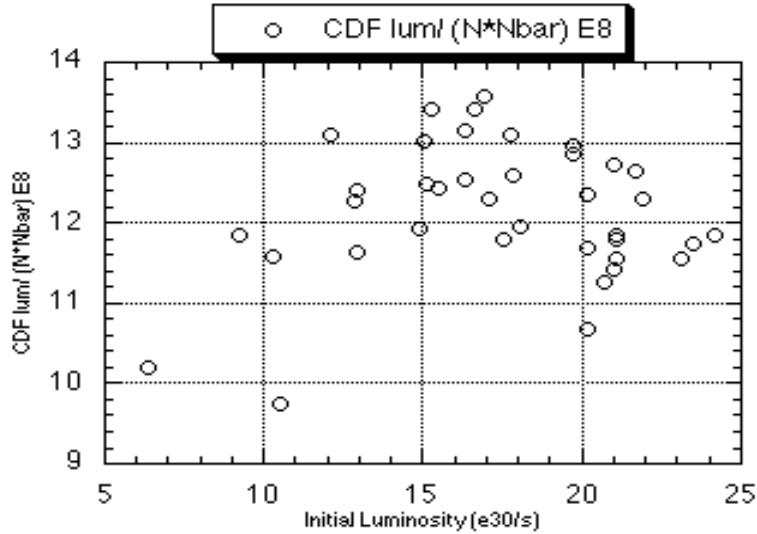
Figure 24 CDF \mathcal{L}/(N_p N_{\bar{p}}) for Recent Stores (Stores 5562-5629)
