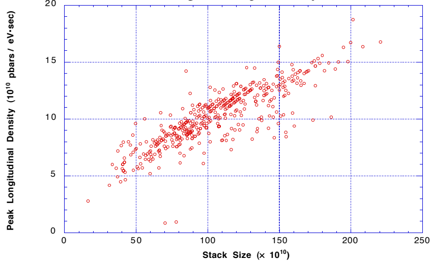
Figure 7. Longitudinal phase space density at the peak of the antiproton momentum distribution just prior to unstacking as a function of stack size.
