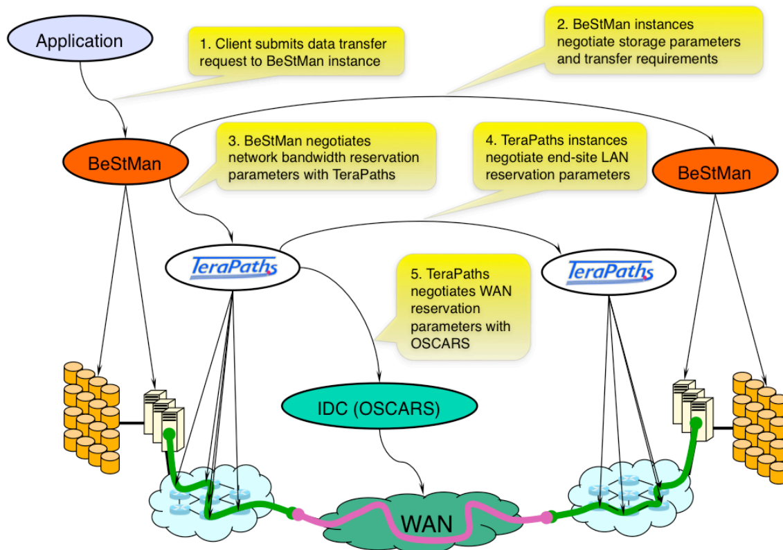
Figure 1: StorNet workflow
