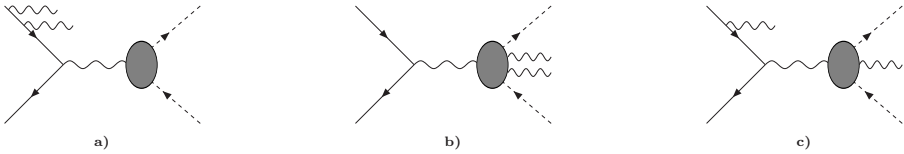
Fig. 3. The classes of diagrams with the emission of two photons, which contribute to the radiative return cross section at the NLO. The \pi^+\pi^- final state is assumed and blob represents modeling of the pion-antipion-photon interaction.
