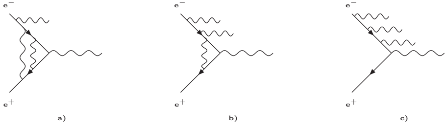
Fig. 4. Possible contributions to the cross section for the reaction e^+e^- \rightarrow \gamma^*(Q^2) + \gamma at the NNLO.
