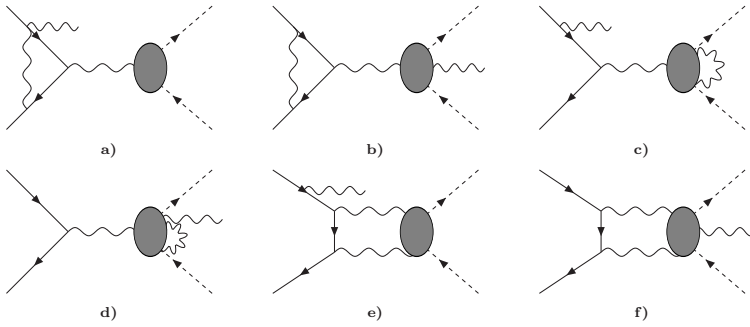
Fig. 2. The classes of virtual corrections, which contribute to the reaction e^+e^- \rightarrow f(Q^2) + \gamma at the NLO. The \pi^+\pi^- final state is assumed and blob represents modeling of the pion-antipion-photon interaction.
