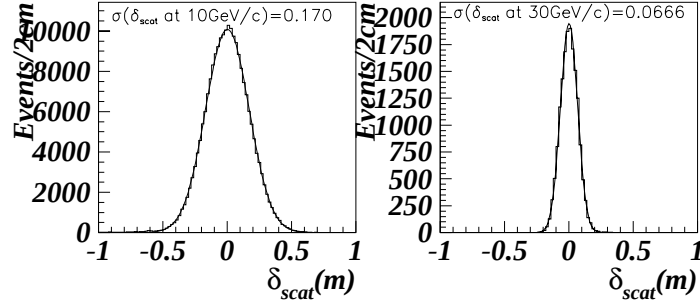
Figure B.1: The \delta_{scat} distribution. The left plot shows the distribution for 10~11GeV/c muons. The right plot shows the distribution for 30~31GeV/c.
