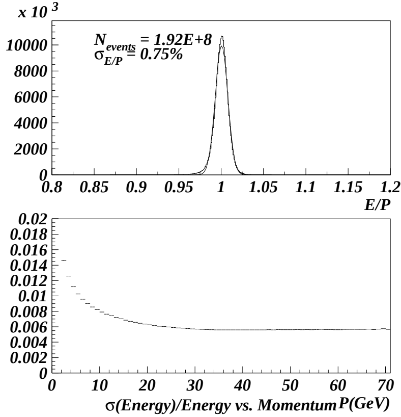
Figure 2.6: The upper plot shows the E/P distribution for electrons in K_L \rightarrow \pi e \nu , where E denotes an measured energy by the calorimeter, and P represents a measured momentum by the spectrometer. The lower plot shows the intrinsic energy resolution of the calorimeter as a function of electron momentum.
