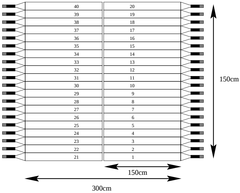
Figure 2.9: The upper figure shows MU3x bank. The lower figure illustrates MU3y bank.
