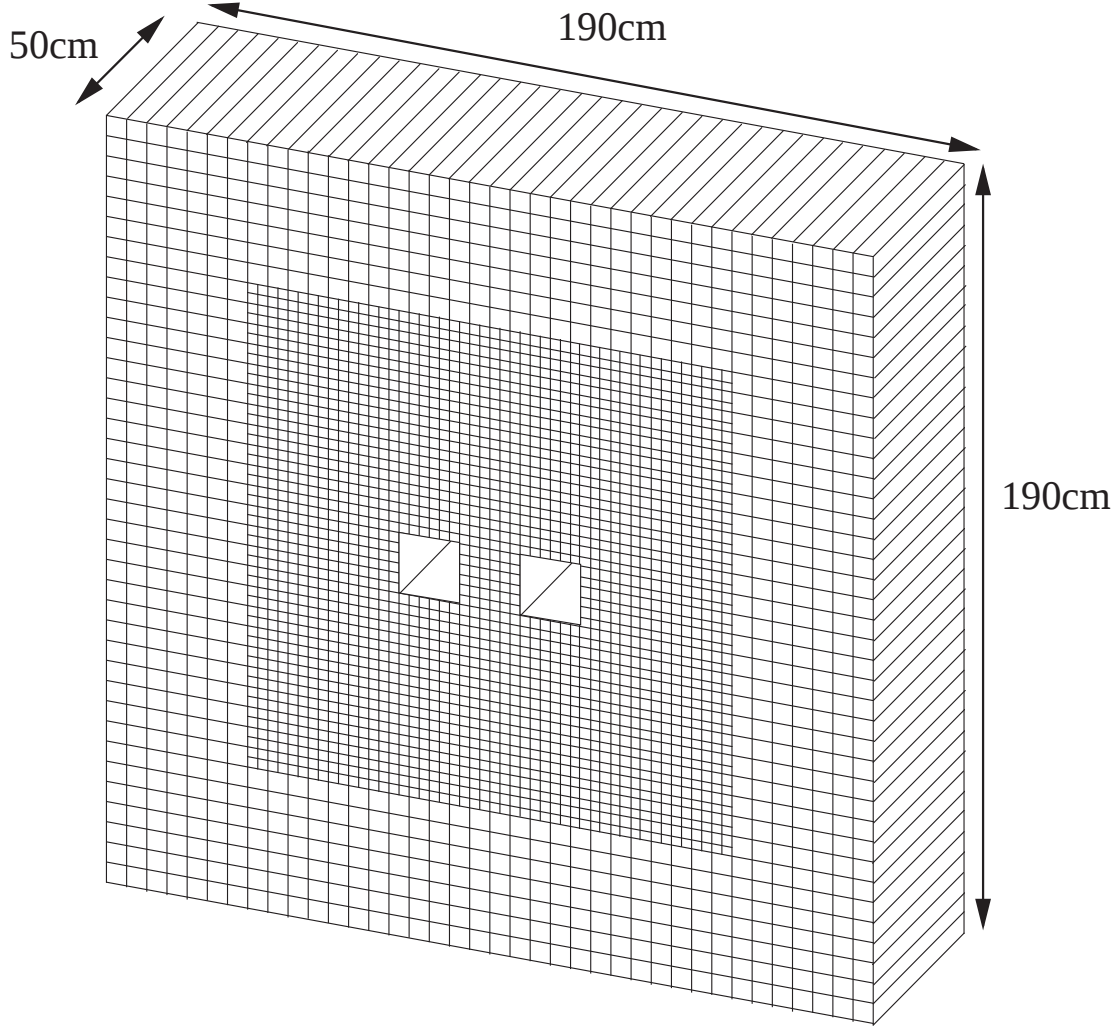
Figure 2.7: Pure-CsI Electromagnetic Calorimeter
