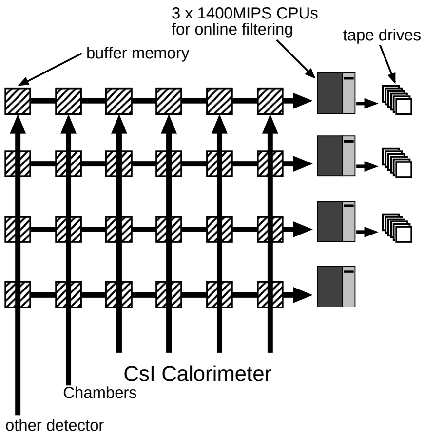
Figure 2.10: KTeV Data Acquisition System
