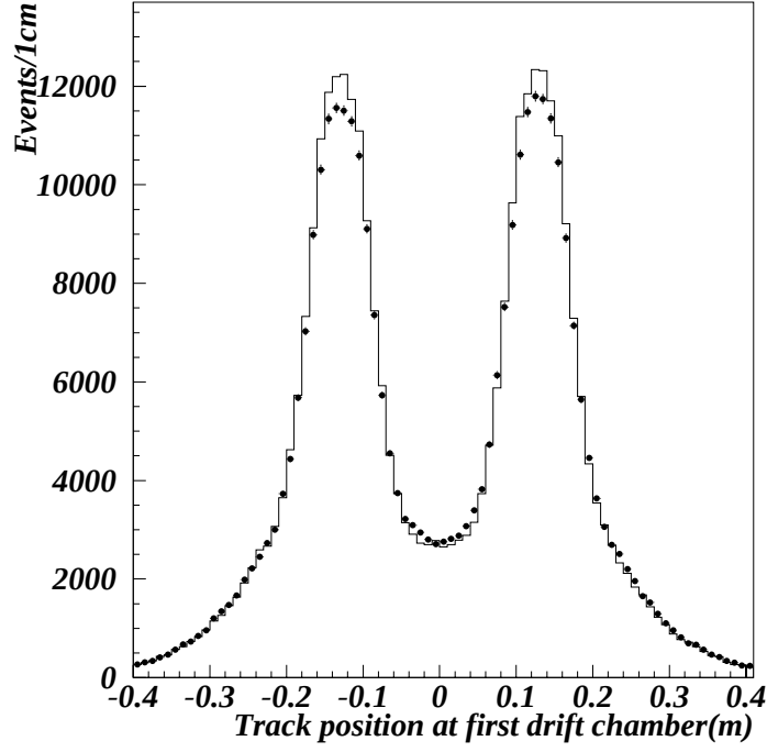
Figure 6.1: The illumination of the tracks at the first drift chamber.
