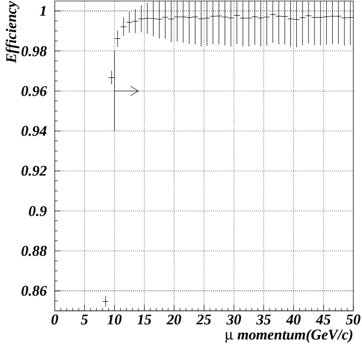
Figure 4.4: The efficiency for detecting muons by MU3x bank as a function of its momentum. We required more than 10GeV/c for muon momentum as shown by arrow in the plot.
