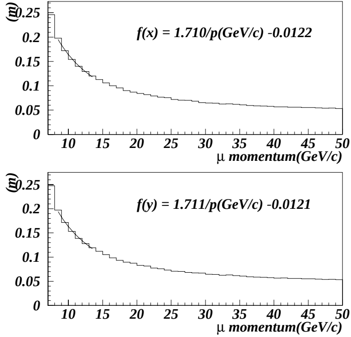
Figure B.2: The \delta_{scat} distribution as a function of the muon momentum. The upper plot shows the distribution for x direction. The lower plot shows the distribution for y direction.
