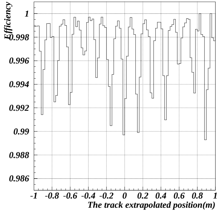
Figure 4.12: The detection efficiency of MU3 bank for muons as a function of the extrapolated track position at MU3x bank. The muons were selected to have momentum to be greater than 40\text{GeV}/c .
