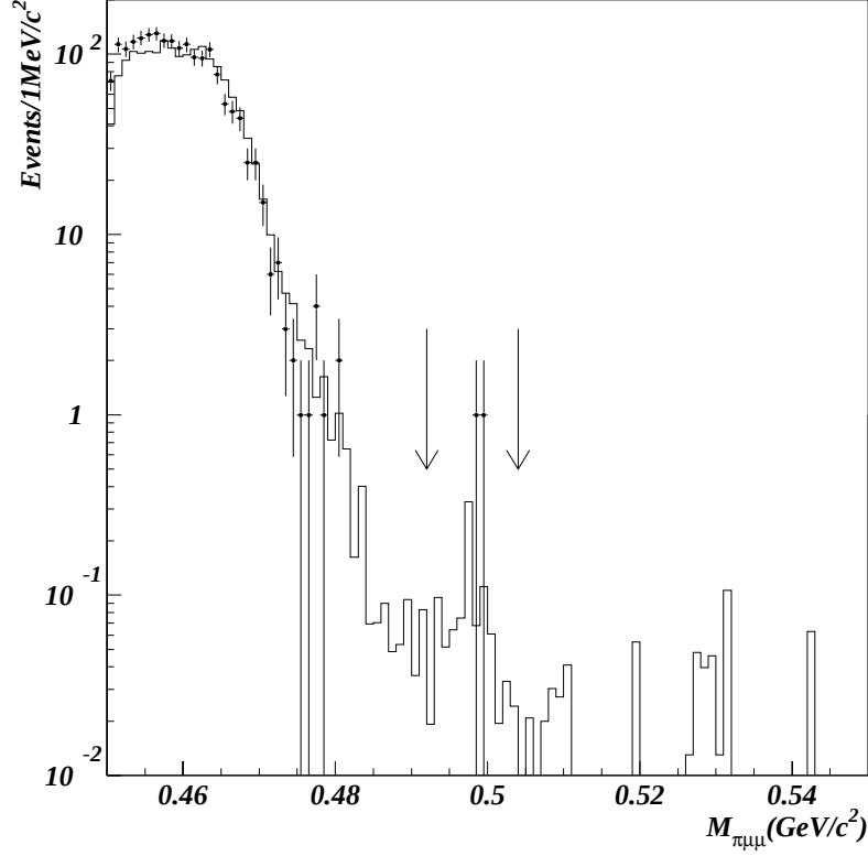
Figure 7.1: The reconstructed \pi^0\mu^+\mu^- mass distribution with all the cuts except for the mass cut. There are two events in the masked region. Dots are data. Open histogram is sum of all background MC events.
