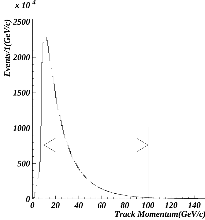
Figure 4.5: The \mu momentum distribution of the K_L \rightarrow \pi^0 \mu^+ \mu^- for the K_L \rightarrow \pi^0 \mu^+ \mu^- trigger events after the event reconstruction. We required the momentum to be greater than 10 GeV/c and less than 100 GeV/c as shown by arrow in the plot.
