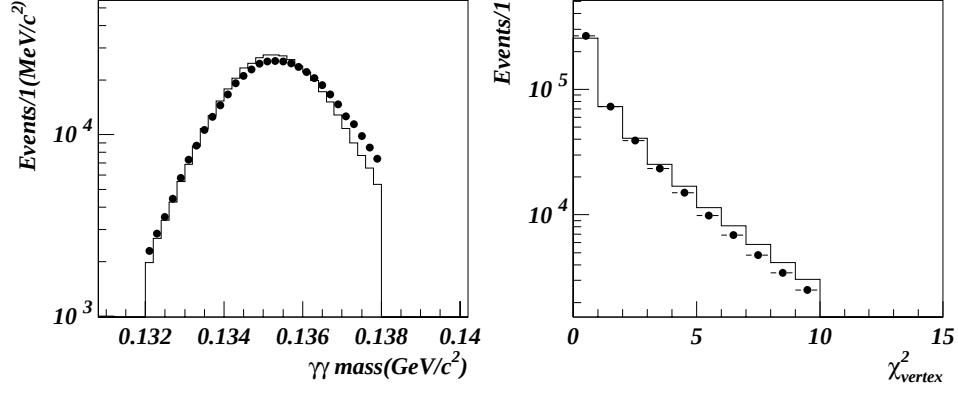
Figure 4.14: The left plot shows \gamma\gamma mass distribution of data(dot) and MC(open histogram) of the accepted K_L \rightarrow \pi^0 \pi^+ \pi^- events as normalization. The right plot shows \chi^2_{vertex} distribution of data(dot) and MC(open histogram).
