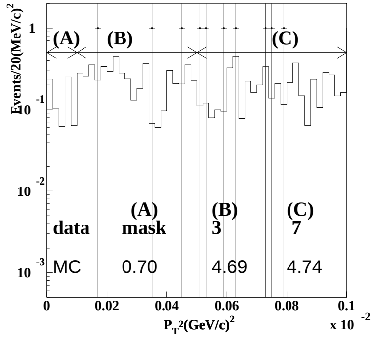
Figure A.8: The P_T^2 distribution in the kaon mass region. The dots indicate data. The open histogram represents the summed MC.
