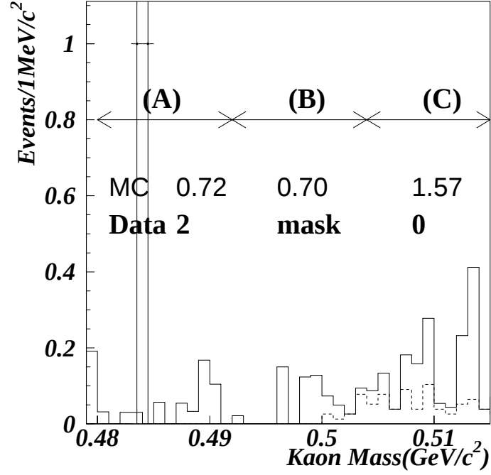
Figure A.7: The kaon mass distribution in the P_T^2 < 100 (MeV/c)^2 region. The dot indicates the data. The open histogram represents the summed MC. The dashed line shows the contribution from K_L \rightarrow \mu^+ \mu^- \gamma + \gamma_{acc} . Most of the other contribution is from K_L \rightarrow \pi^\pm \mu^\mp \nu(\bar{\nu}) + 2\gamma_{acc} .
