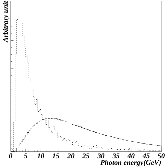
Figure A.1: The energy distribution of the photon in the K_L \rightarrow \mu^+ \mu^- \gamma (solid) and the accidental photon(dot).
