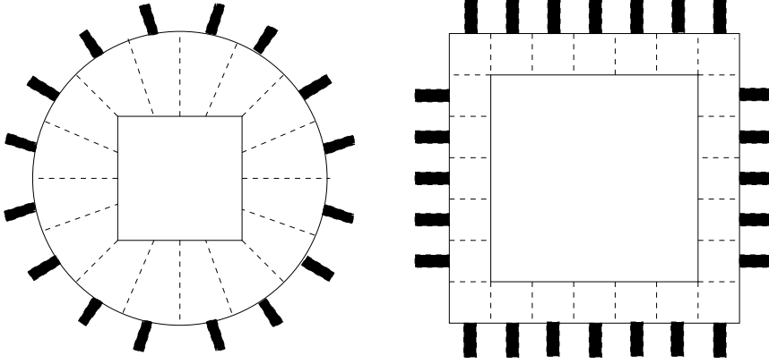
Figure 2.3: The photon veto detectors. The left figure shows a RC which was located inside the vacuum region. The right figure shows the SA and CIA.
