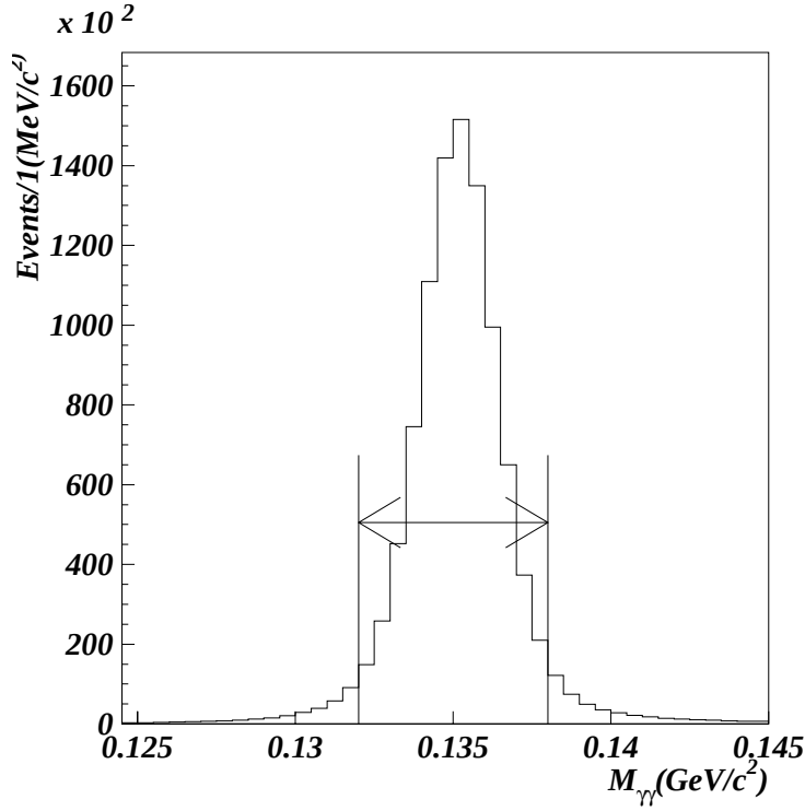
Figure 4.7: The \pi^0 distribution of the K_L \rightarrow \pi^0 \mu^+ \mu^- MC after the event reconstruction. The arrow in the plot shows our requirement ( 132 < M_{\gamma\gamma} \text{ MeV}/c^2 < 138 ).
