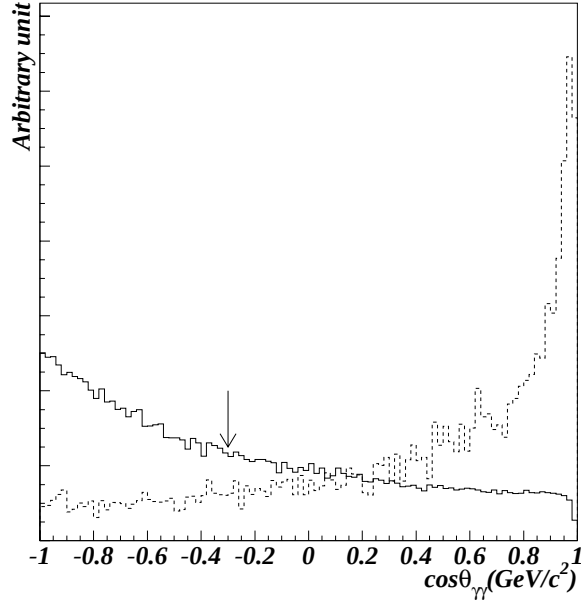
Figure A.6: The \cos\theta_{\gamma\gamma} distribution of K_L \rightarrow \mu^+\mu^-\gamma\gamma and K_L \rightarrow \pi^\pm\mu^\mp\nu(\bar{\nu}) . The solid(dashed) line represents the distribution for K_L \rightarrow \mu^+\mu^-\gamma\gamma(K_L \rightarrow \pi^\pm\mu^\mp\nu(\bar{\nu})) after P_{\pi^0}^2 cut. The arrow shows our requirement.
