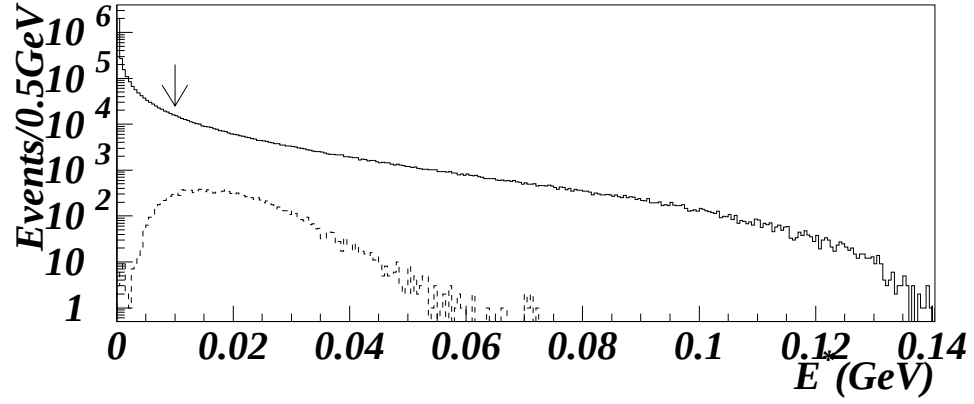
Figure A.10: The spectrum of the minimum energy photon in our K_L \rightarrow \mu^+ \mu^- \gamma \gamma MC events. The solid line shows the spectrum at the generation. The dashed line shows the spectrum for the accepted events. The arrow shows the cutoff which was used to calculate the branching ratio.
