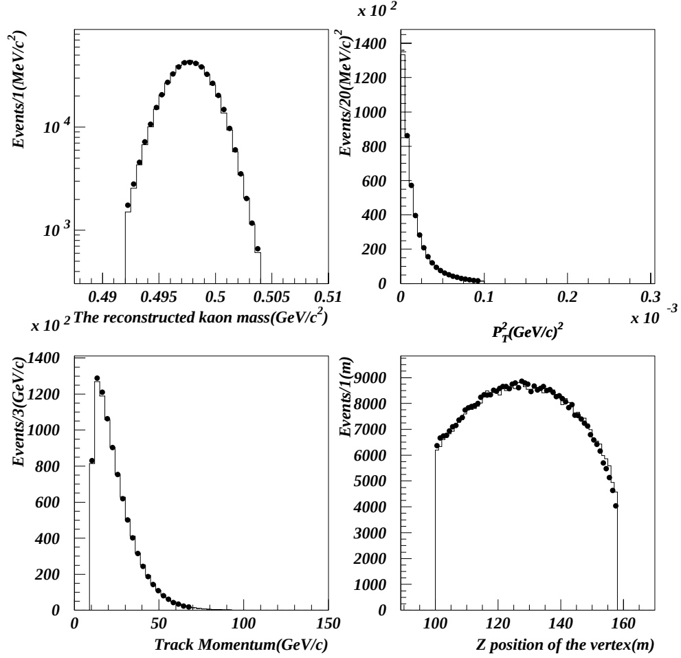
Figure 4.13: The top left(right) plot shows the kaon mass( P_T^2 ) distribution of K_L \rightarrow \pi^0 \pi^+ \pi^- MC events and data after all cuts. The bottom left plot shows the momentum distribution of the track in the K_L \rightarrow \pi^0 \pi^+ \pi^- events. The bottom right plot shows the vertex z position. Dots represent the distribution of the observed events. Open histogram shows that of MC events. The MC distribution was normalized by the measured number of decayed K_L .
