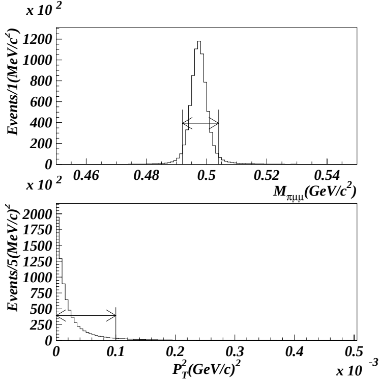
Figure 4.10: The upper plot shows the reconstructed \pi^0\mu^+\mu^- mass distribution. The lower plot shows P_T^2 of K_L \rightarrow \pi^0\mu^+\mu^- MC events after the event reconstruction. The arrow in these plots shows our requirement. ( 492 < M_{\pi^0\mu^+\mu^-} \text{ MeV}/c^2 < 504 , P_T^2 < 100 (\text{MeV}/c)^2 )
