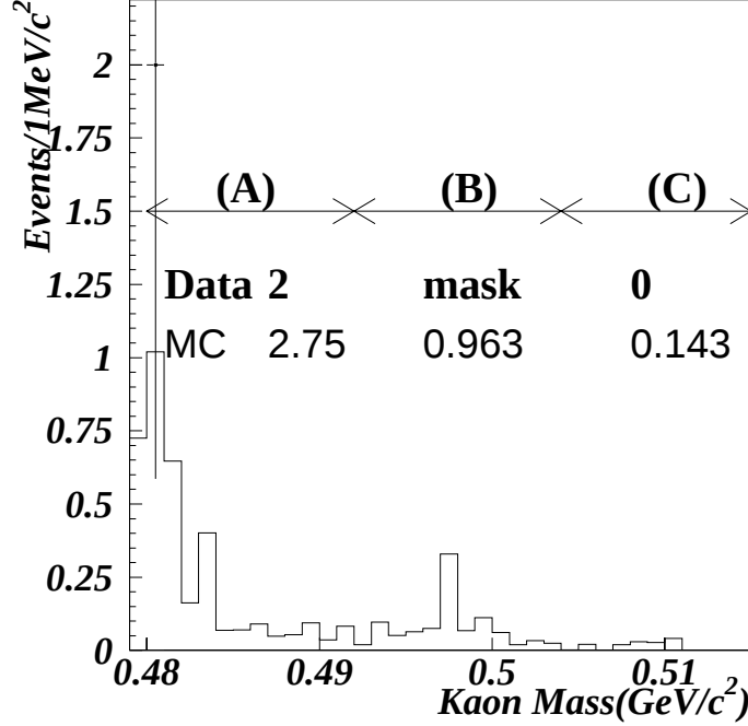
Figure 5.2: The kaon mass distribution in the P_T^2 < 100 (MeV/c)^2 region. The dot indicates the data. The open histogram represents the summed MC.
