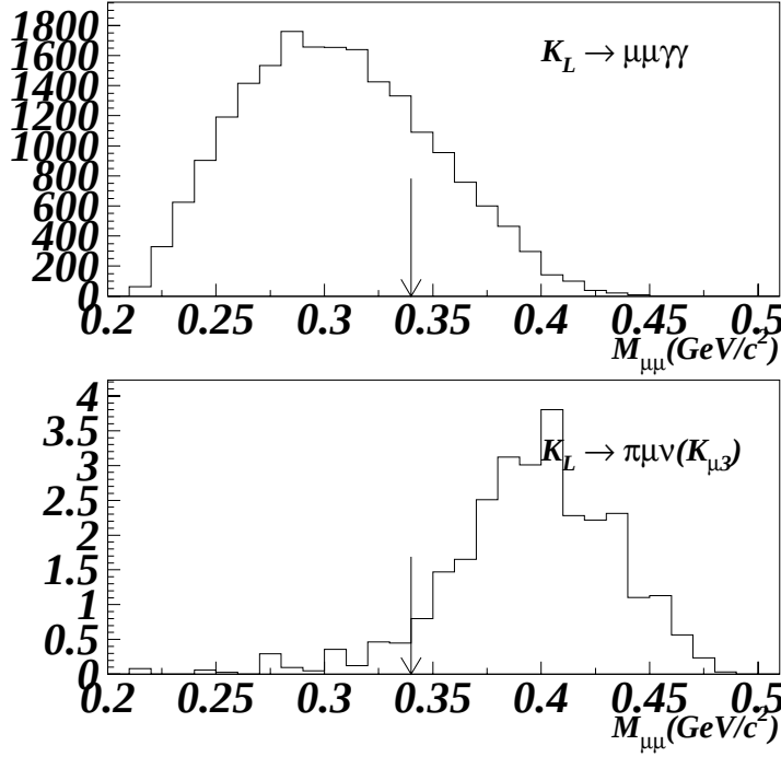
Figure A.4: M_{\mu\mu} distribution for each decay after the \pi^0 mass cut. The upper plot shows the distribution for the K_L \rightarrow \mu^+\mu^-\gamma\gamma . The lower plot shows the distribution for the K_L \rightarrow \pi^\pm\mu^\mp\nu(\bar{\nu}) . We required M_{\mu\mu} < 0.34\text{GeV}/c^2 as indicated by the arrow.
