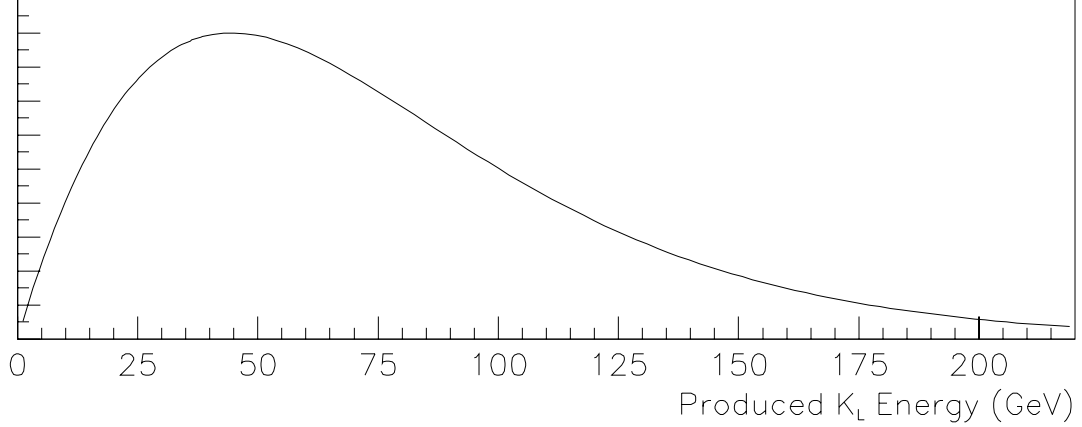
Figure 2.1: The energy spectrum of the kaon at the target
