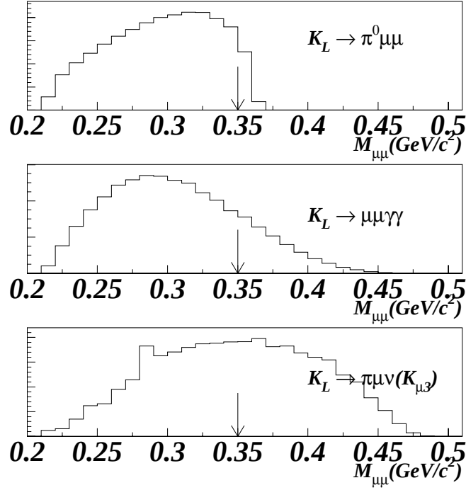
Figure 4.8: M_{\mu\mu} distribution for each decay after the \pi^0 mass cut. The upper plot shows distribution of K_L \rightarrow \pi^0 \mu^+ \mu^- . The middle plot shows the distribution of the K_L \rightarrow \mu^+ \mu^- \gamma \gamma . The lower plot shows the distribution of the K_L \rightarrow \pi^\pm \mu^\mp \nu(\bar{\nu}) . We required M_{\mu\mu} < 0.35 \text{ GeV}/c^2 as indicated by the arrow.
