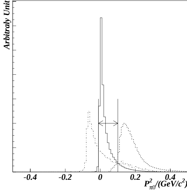
Figure 4.9: The P_{\pi^0}^2 distribution after M_{\mu\mu} cut for K_L \rightarrow \pi^0 \mu^+ \mu^- (solid line), K_L \rightarrow \pi^0 \pi^+ \pi^- (dashed line), K_L \rightarrow \pi^\pm \mu^\mp \nu(\bar{\nu}) (dotted line), and K_L \rightarrow \mu^+ \mu^- \gamma\gamma (dot-dash line) as normalized by area.
