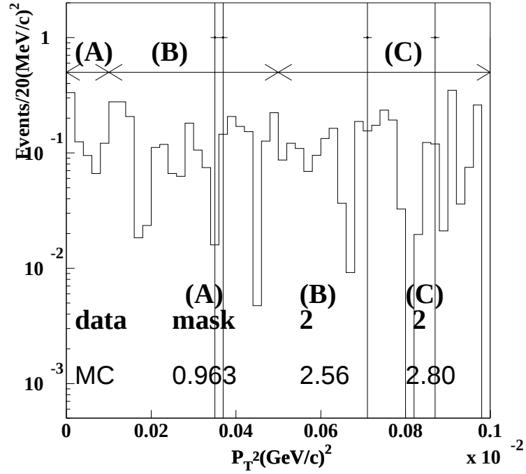
Figure 5.3: The P_T^2 distribution in the kaon mass region. The dots indicate data. The open histogram represents the summed MC.
