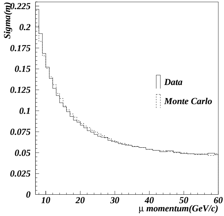
Figure B.3: The \delta_{scat} distribution as a function of \mu momentum for data(solid) and MC(dash) in K_L \rightarrow \pi^\pm \mu^\mp \nu(\bar{\nu}) decays.
