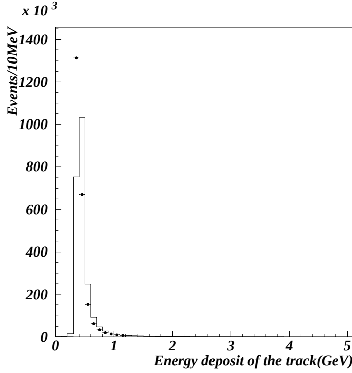
Figure 4.11: The muon energy deposit in the CsI calorimeter. The solid line(dot) shows the energy deposit by muon in MC sample(data).
