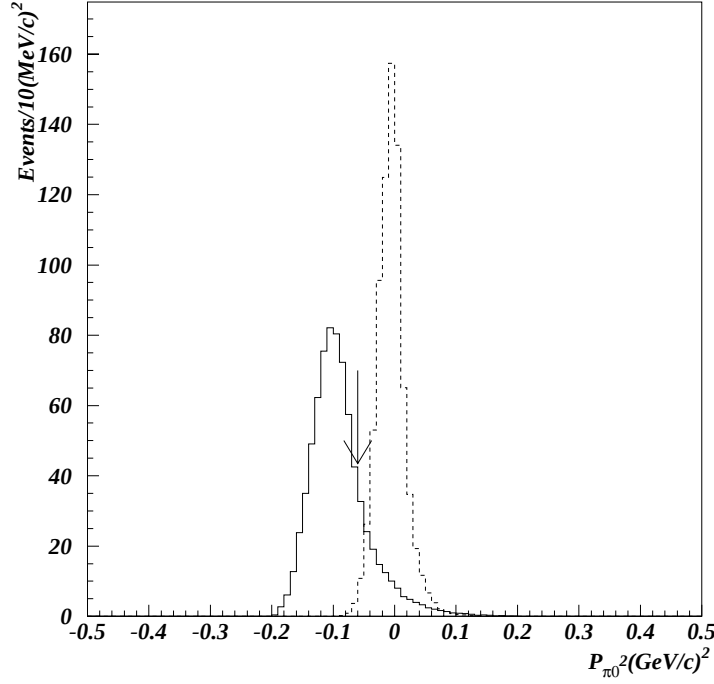
Figure A.3: P_{\pi^0}^2 distribution for K_L \rightarrow \mu^+ \mu^- \gamma \gamma (solid line) and K_L \rightarrow \pi^0 \pi^+ \pi^- (dashed line) which include both \pi^\pm decayed in flight. We required the P_{\pi^0}^2 to be less than -0.06 as indicated arrow in the plot. The distributions are normalized by area.
