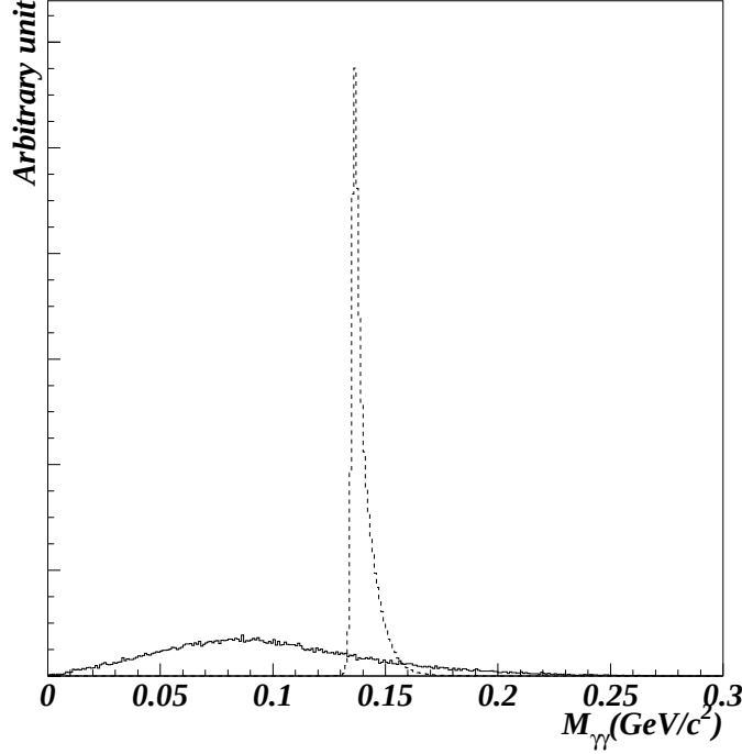
Figure A.2: The \pi^0 distribution of the K_L \rightarrow \mu^+ \mu^- \gamma \gamma MC events(solid line) and K_L \rightarrow \pi^0 \pi^+ \pi^- MC events(dash line) after particle identification. These distributions are normalized by area.
