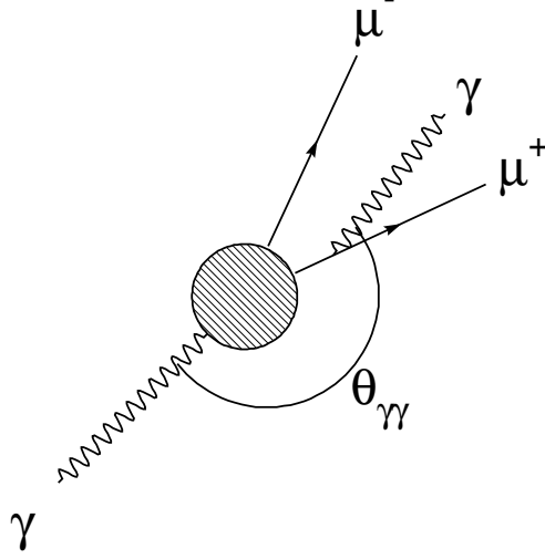
Figure A.5: The illustration showing the angle between two photons in the center of mass system.
