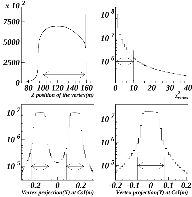
Figure 4.2: The distributions for the vertex variables for the K_L \rightarrow \pi^0 \mu^+ \mu^- after the vertex reconstruction. The top left plot shows the Z distribution of the reconstructed vertex. The top right plot shows the \chi_{vertex}^2 distribution. The bottom plots show the projected position of the vertex from the target to the CsI calorimeter. The bottom left(right) plot shows the X(Y) distribution of the projection. The arrows in the plots show our requirements for the vertex.
