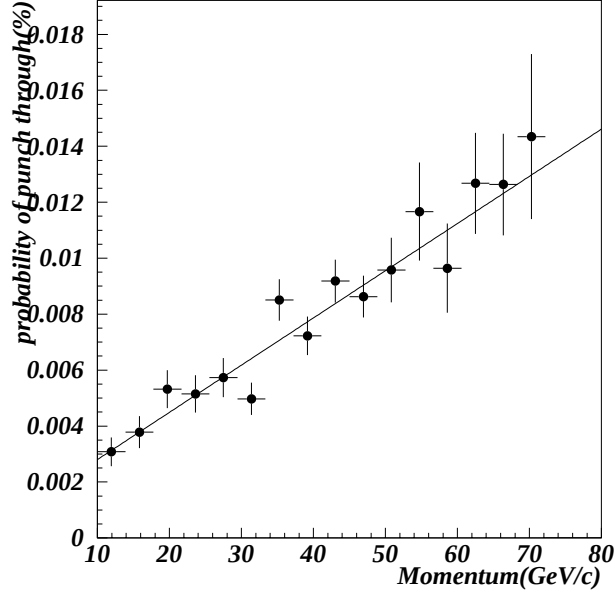
Figure 3.1: The \pi^\pm punch through probability as a function of \pi^\pm momentum, obtained by GEANT simulation. The line shows the result from the linear fit.
