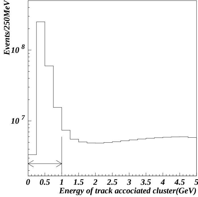
Figure 4.3: The energy distribution of the cluster associated with a track at CsI calorimeter for K_L \rightarrow \pi^0 \mu^+ \mu^- trigger events.
