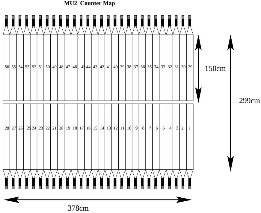
Figure 2.8: The MU2 bank.
