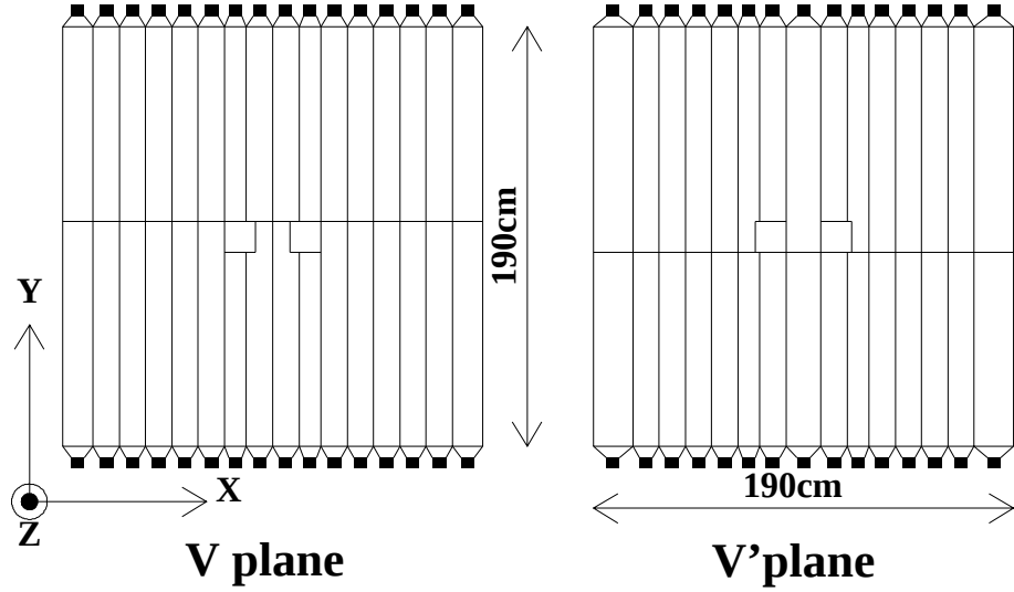
Figure 2.5: Schematic view of Trigger Hodoscopes(V, V' bank).
