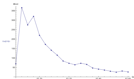
Figure 5: Particle losses through the 18 GeV RCS acceleration cycle as a function of horizontal tune. The initial bunch parameters were RMS dp/p = 4.3e-3 , and bunch length of 71 ps RMS.
