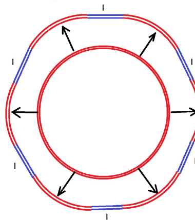
Figure 3: Projecting the pure ring lattice with 96 super-periodicity onto the RHIC six fold periodic ring.
