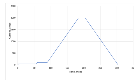
Figure 2: Power supply profile of RCS Ramp.
