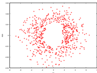
Figure 4: RCS lattice Phase space plot of dp/p and cm showing lost particles over 200 turns.
