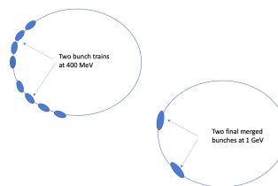
Figure 6: 8 bunches injected into two trains of four bunches in the RCS at 400 MeV. (left plot). Bunches merge at 1 GeV into two bunches.
