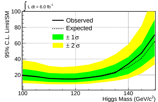
FIG. 3: Expected (dashed curve) and observed (solid curve) 95% C.L. upper limit on \sigma(p\bar{p} \rightarrow H)B(H \rightarrow \tau\tau) , as a function of the mass, in the range between 100 and 150 \text{GeV}/c^2 .
