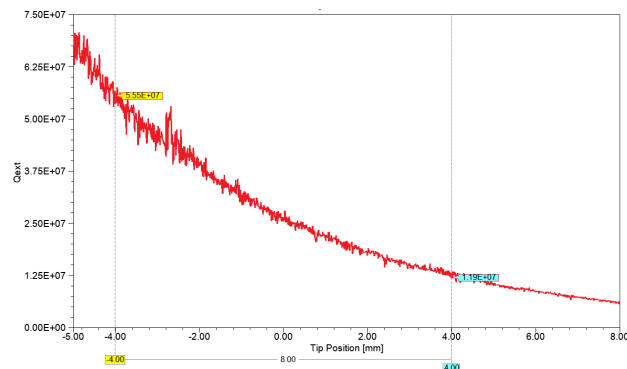
Figure 4: The Q_{\text{ext}} range achievable with a tip length of 333.9 mm and a range of movement of \pm 4 mm.
