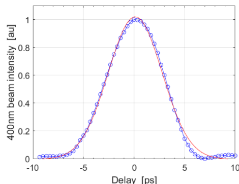
Figure 4: Measurement result for UV pulse duration.
