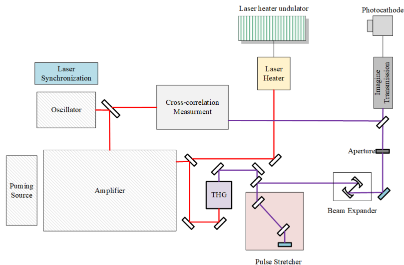
Figure 1: Schematic of SXFEL drive laser system.
