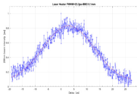
Figure 5: Measurement result for Laser heater pulse duration.
