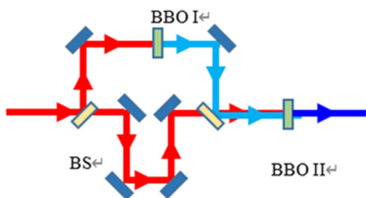
Figure 2: Schematic of the THG.
