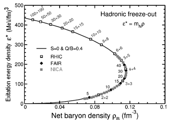
Fig. 1. Freeze-out diagram for baryonic matter showing baryon density reachable at different facilities both in collider and fixed target experiments [4].
