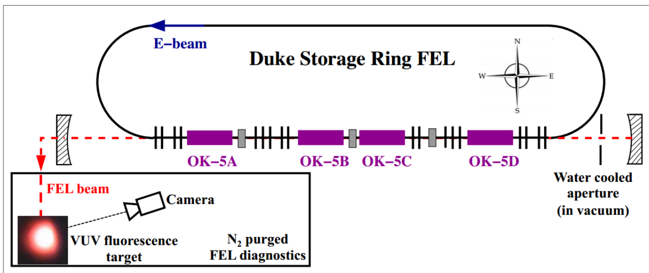
Figure 5: Configuration of the OK-5 FEL for production of high energy gamma-ray beams using VUV mirrors. OK-5A, OK-5B, and OK-5C were energized for the 86 MeV and 120 MeV gamma-ray beam production using 175 nm mirrors.
