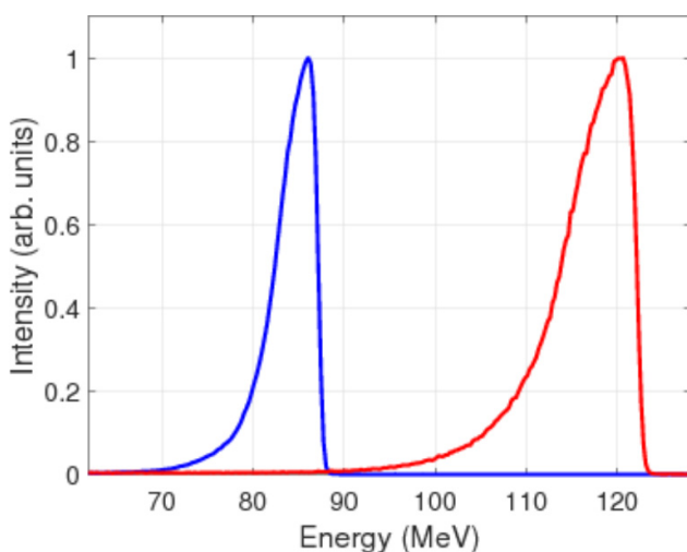
Figure 6: Energy spectra of 86 MeV and 120 MeV gamma-ray beams produced using 0.936 GeV and 1.11 GeV electron beams. The gamma-ray spectra are measured using a high-resolution NaI detector, and normalized to their respective peak intensity.
