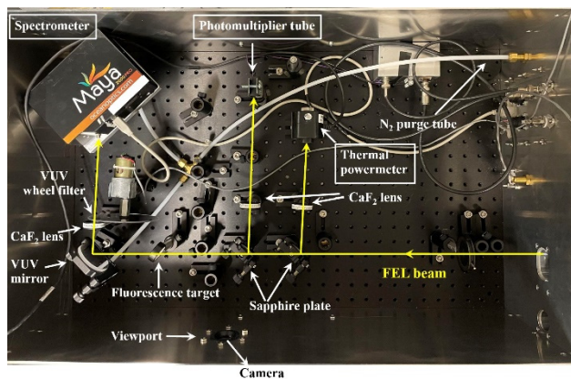
Figure 2: VUV optical diagnostics board.
