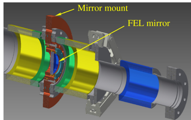
Figure 3: Copper mirror holder and mount for downstream FEL mirror.
