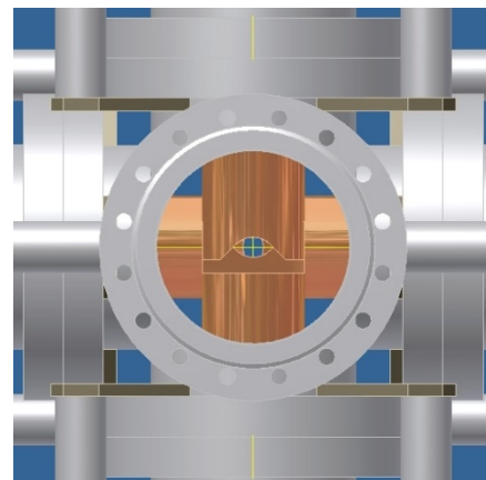
Figure 4: In-vacuum mirror protection water-cooled horizontal and vertical apertures in fully inserted position.
