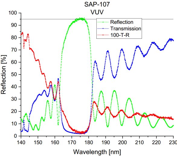
Figure 1: Measured reflectivity and transmission of a new 175 nm fluoride FEL mirror (serial number SAP-107) used at the downstream side of the optical FEL cavity during the first 120 MeV HIGS user run.
