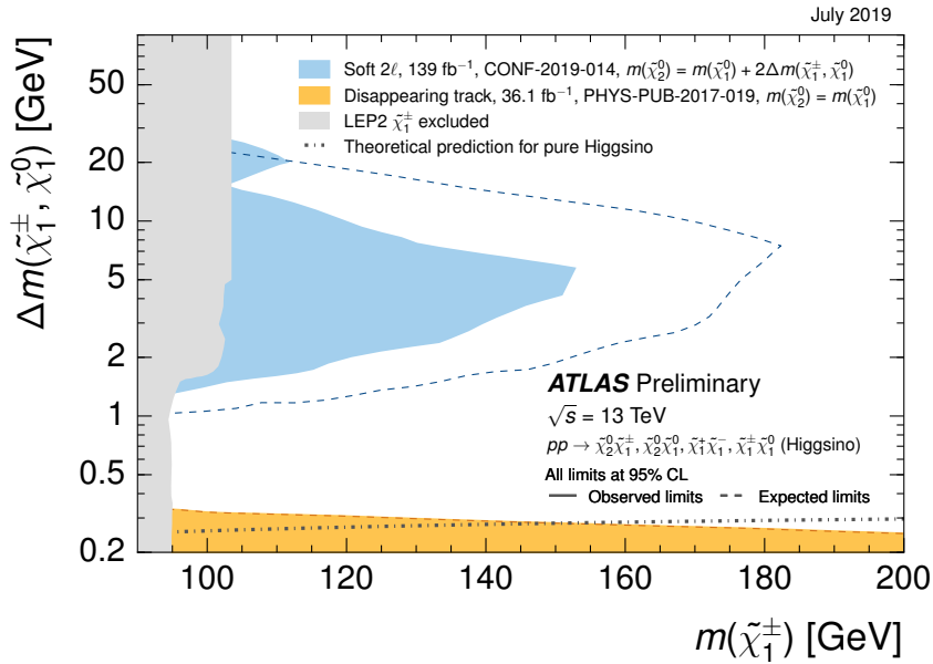
Figure 17: Exclusion limits at 95% CL for higgsino pair production \tilde{\chi}_1^+ \tilde{\chi}_1^- , \tilde{\chi}_1^\pm \tilde{\chi}_1^\pm , \tilde{\chi}_1^\pm \tilde{\chi}_2^0 , and \tilde{\chi}_1^0 \tilde{\chi}_2^0 with off-shell SM-boson-mediated decays to the lightest neutralino, \tilde{\chi}_1^0 , as a function of the \tilde{\chi}_1^\pm and \tilde{\chi}_1^0 masses. The production cross-section is for pure higgsinos.
