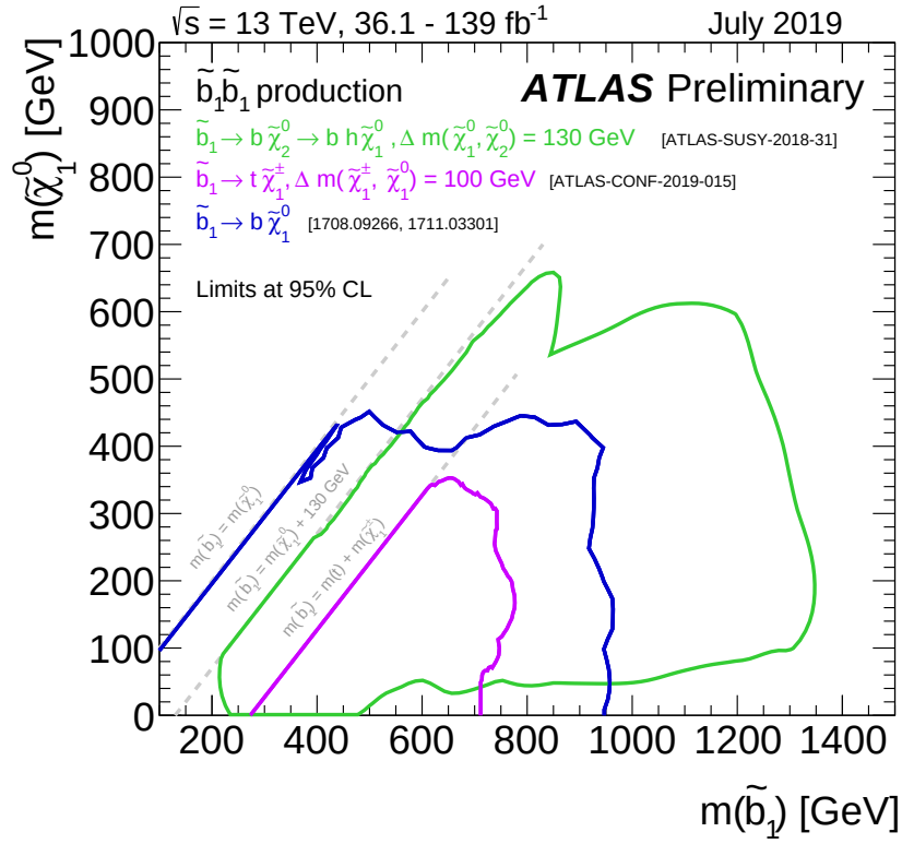
Figure 11: Exclusion limits at 95% CL in the (lightest sbottom, lightest neutralino) mass plane for direct sbottom production. The lightest neutralino ( \tilde{\chi}_1^0 ) is assumed to be the lightest SUSY particle (LSP). Several different decay scenarios are shown, along with different parameterizations of the intermediate particles in the models.
