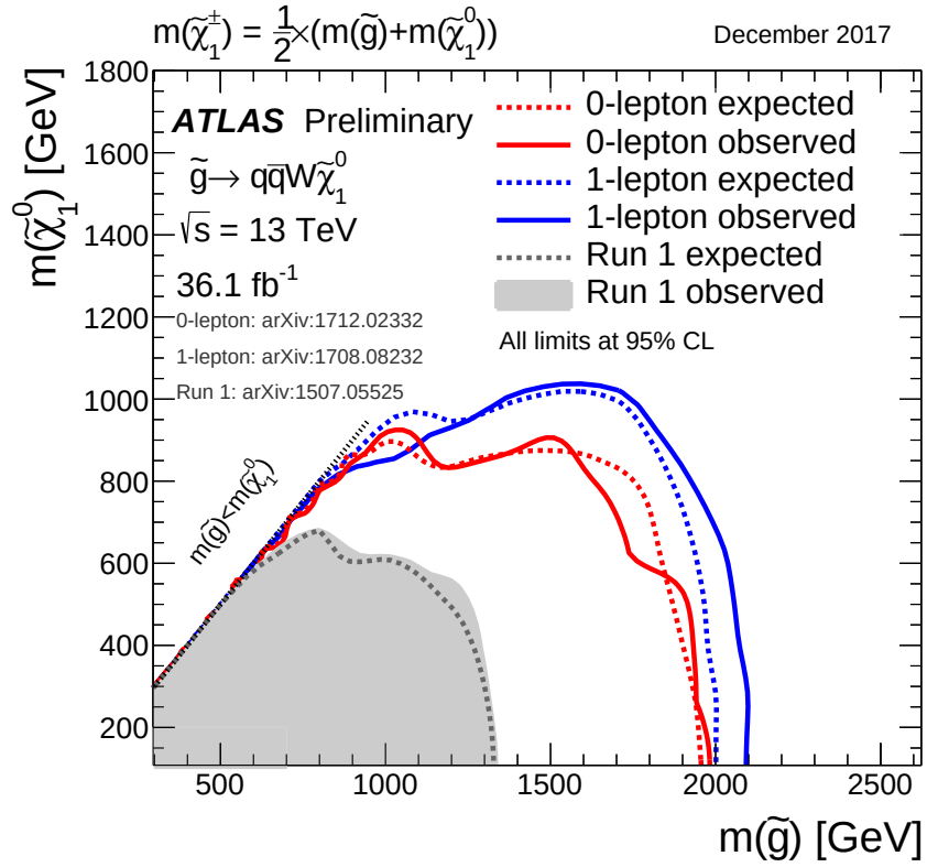
Figure 4: Exclusion limits at 95% CL based on 13 TeV data in the (gluino, lightest neutralino) mass plane for the simplified model where a pair of gluinos are produced, and each decays promptly via an on-shell chargino to a pair of quarks, a W boson, and the lightest neutralino. The chargino mass is assumed to be mid-way between the gluino and neutralino masses. Theoretical signal cross section uncertainties are not included in the limits shown.
