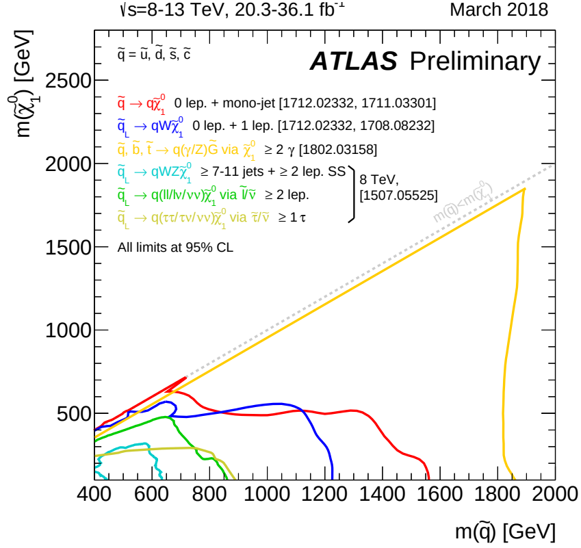
Figure 2: Exclusion limits at 95% CL based on 8 and 13 TeV data in the (squark, lightest neutralino) mass plane for different simplified models featuring the decay of squarks to the lightest supersymmetric particle (lightest neutralino or gravitino) either directly or through a cascade chain featuring other SUSY particles with intermediate masses. For each line, the squark decay mode is reported in the legend and it is assumed to proceed with 100% branching ratio. Some limits depend on additional assumptions on the mass of the intermediate states, as described in the references provided in the plot.
