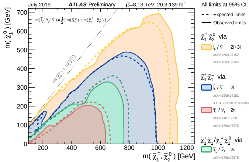
Figure 13: The 95% CL exclusion limits on \tilde{\chi}_1^\pm \tilde{\chi}_1^\mp and \tilde{\chi}_1^\pm \tilde{\chi}_2^0 production with \tilde{\ell} -mediated decays, as a function of the \tilde{\chi}_1^\pm , \tilde{\chi}_2^0 and \tilde{\chi}_1^0 masses. The production cross-section is for pure wino \tilde{\chi}_1^\pm \tilde{\chi}_1^\mp and \tilde{\chi}_1^\pm \tilde{\chi}_2^0 . Each individual exclusion contour represents a union of the excluded regions of one or more analyses.
