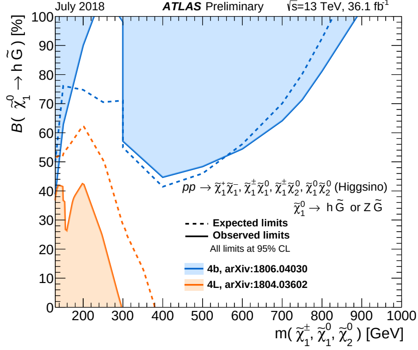
Figure 18: The 95% CL exclusion limits on a general gauge mediation model from 13 TeV data. The model assumes a pure Higgsino NLSP that promptly decays to either Z gravitino or Higgs gravitino. The limits are displayed as a function of the mass of the nearly mass-degenerate Higgsino triplet and the branching fraction of lightest Higgsino to Higgs gravitino.
