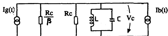
Fig. 3. Equivalent circuit of a cavity with beam. Generator and beam currents I_g(t) , I_b(t) , cavity voltage V_c and resistance R_c , coupling factor \beta .
