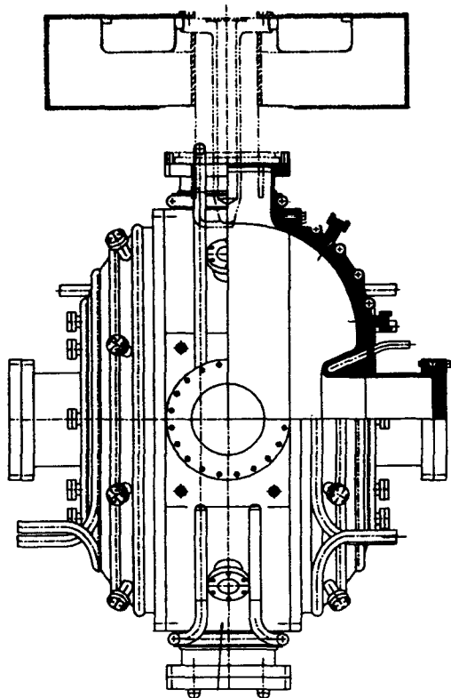
Fig. 1. Cavity for the ANL Advanced Photon Source /10/. Test voltage 1 MV at 352 MHz cw operation.
