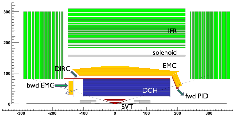
Fig. 2. Concept for the SuperB detector.
