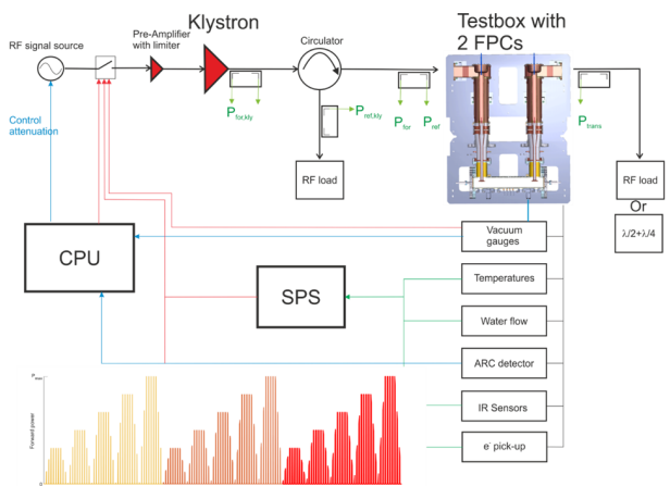
Figure 3: Scheme of the conditioning procedure: The pulse width is increased from a set of power ramps to the next denoted by color code. For each power level a ramping up and back down is performed.
