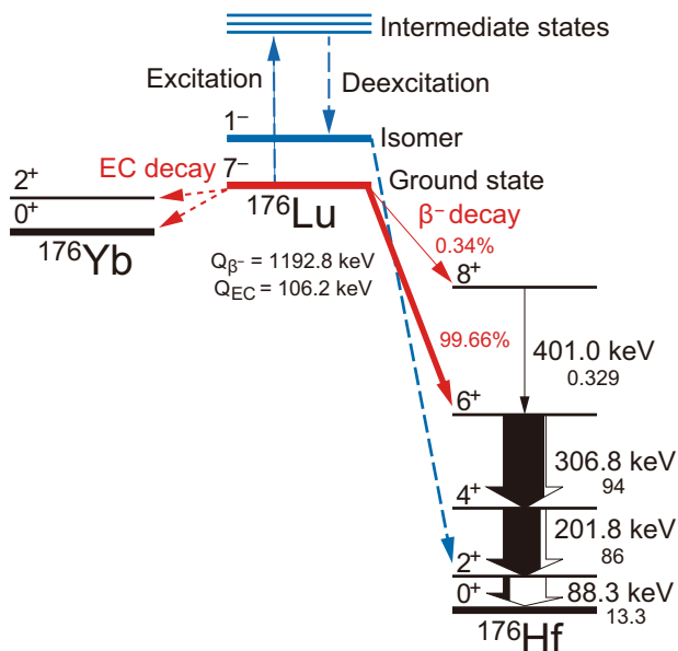
Fig. 1 Partial level scheme of ^{176}\text{Lu} and ^{176}\text{Hf} . The solid area in each arrow and the number below the transition energy indicate the emission probability of the \gamma ray. The blue dashed lines show decay acceleration through the isomer by an incident particle.
