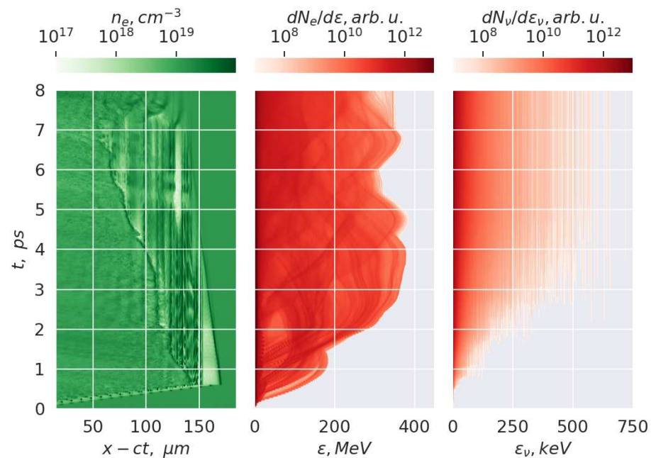
Figure 2. Simulation results for a Gaussian laser pulse with a duration of 11 fs. Spatiotemporal dynamics of electron density at y = 0 ( left ), time dependence of generated electron spectra ( center ), time dependence of generated photon spectra ( right ).
