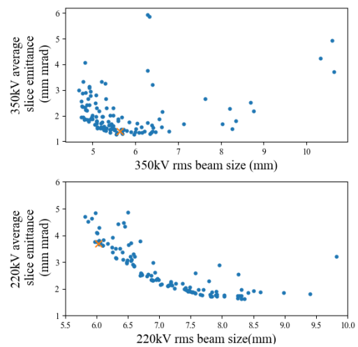
Figure 4: Plots of the objective values of the final solutions showing the average slice emittance against rms beam size for both of the operational voltages. The selected solution is marked as in orange. The x axis of the 220 kV plot is zoomed in for clarity but two solutions with large rms beam size are no longer visible.
