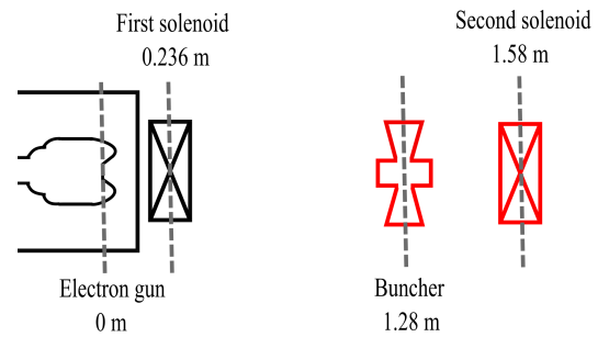
Figure 2: The layout of the start of the PERLE injector. The red elements were not modelled in the optimisation.
