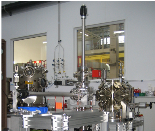
Figure 1: Alkali growth chamber under construction at Daresbury.
