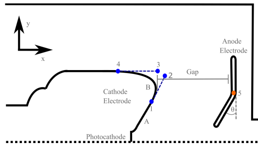
Figure 3: A sketch of the electrode parameterisation. The cathode control points are marked in blue. The dashed dark blue lines show when points are in line. The point where the angled section of the anode begins is marked in orange. The black dashed line is the axis of rotational symmetry.
