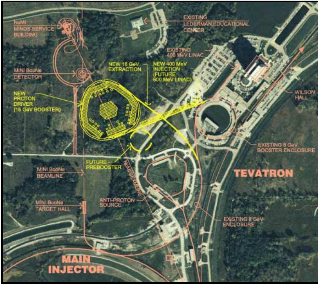
Figure 4.2: FNAL proton driver layout.
