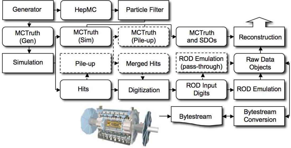
Figure 3.18: Schematic illustration of the ATLAS Simulation framework [88].
