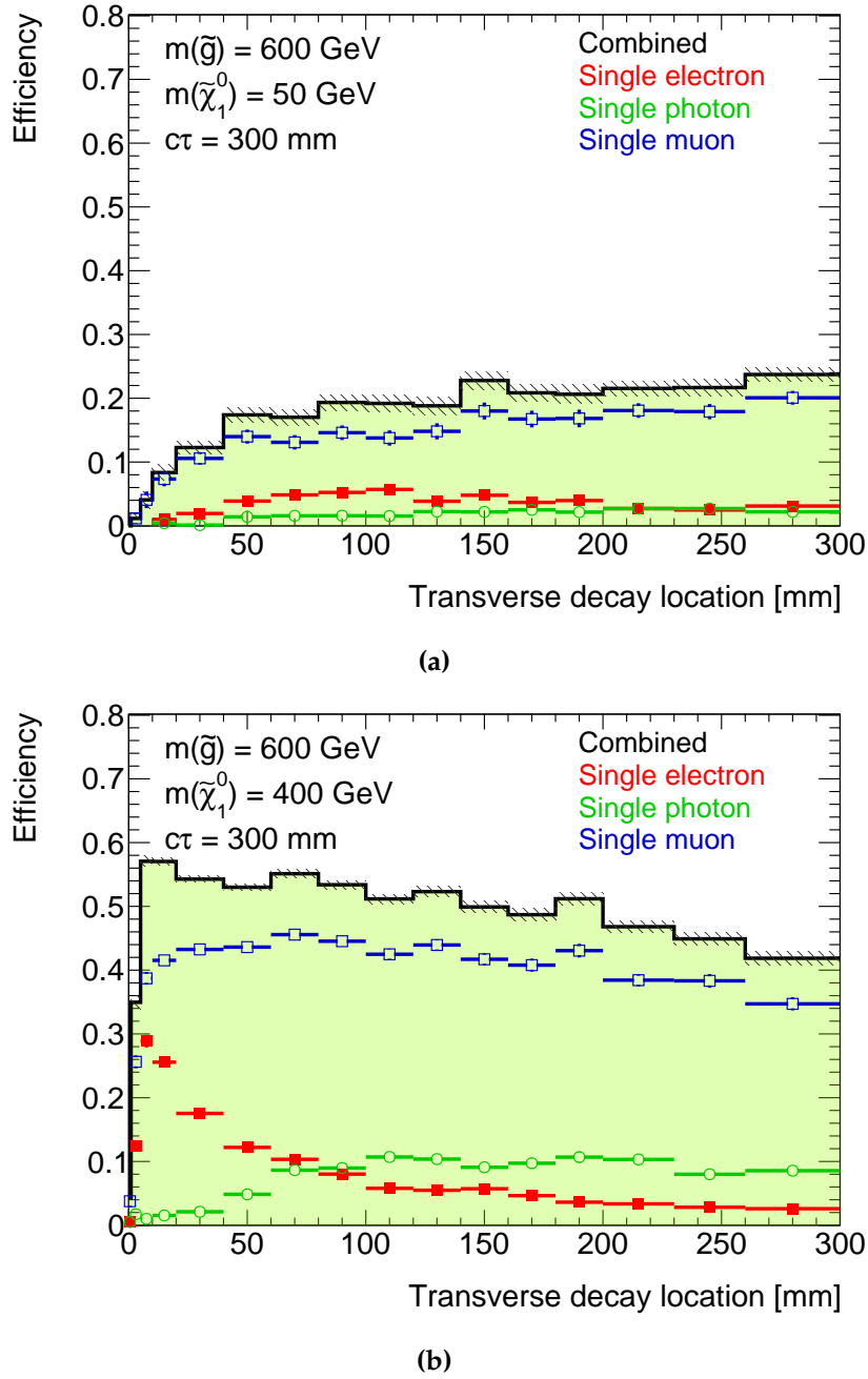
Figure 7.7: Combined and individual trigger and filter efficiencies for individual \tilde{\chi}_1^0 \rightarrow e\mu\nu decays with c\tau = 300 mm in the gluino model for m_{\tilde{g}} = 600 GeV and m_{\tilde{\chi}_1^0} = 50 GeV (a) or m_{\tilde{\chi}_1^0} = 400 GeV (b) as a function of the radial location of the neutralino decay. Statistical errors are given.
