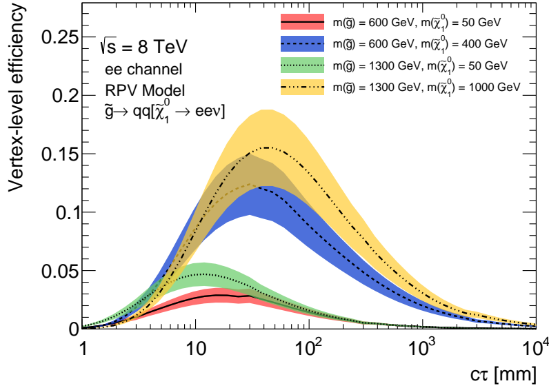
Figure 7.15: Displaced dilepton vertex acceptance times efficiency for \tilde{\chi}_1^0 \rightarrow eev decays as a function of the mean neutralino decay length c\tau for the four NLSP-LSP mass combinations studied. The systematic uncertainties are indicated as coloured bands.
