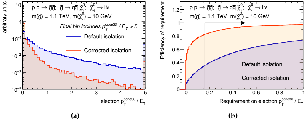
Figure 6.2: Distribution of the electron track isolation variable with (red) and without (blue) correction for nearby leptons (a) and efficiency of the isolation requirements as a function of the cut value (b).
