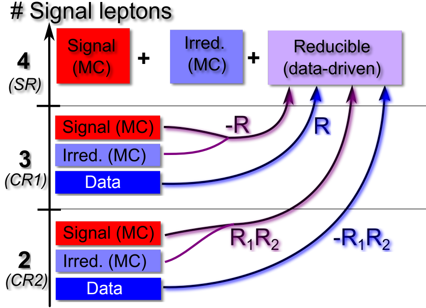
Figure 6.10: Illustration of the weighting technique used to estimate the reducible background in the four-lepton search.
