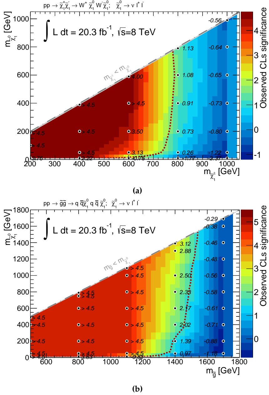
Figure 6.15: Interpolated significance Z_{CL_s} of CL_s and resulting 95% exclusion contour (see text) in the NLSP-neutralino mass plane for the wino (a) and gluino (b) simplified model with \lambda_{121} \neq 0 . The black dots indicate the mass combinations for which CL_s values have been computed.
