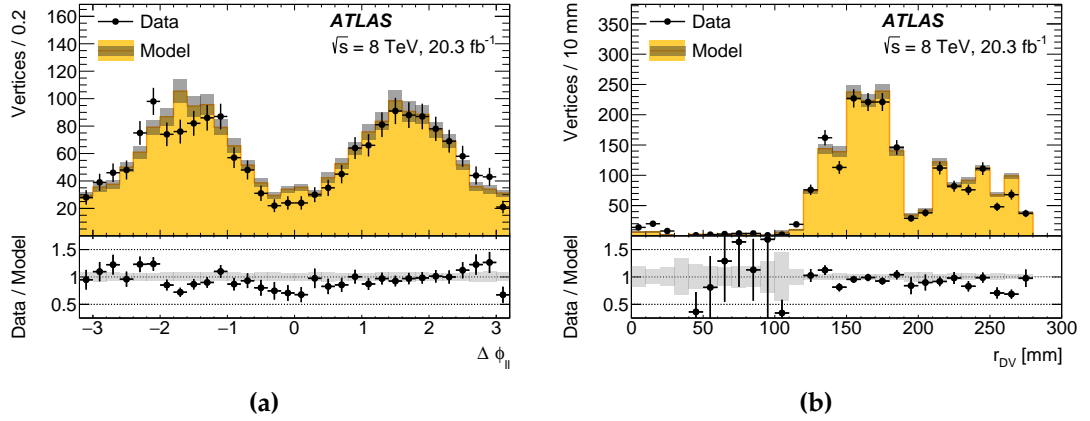
Figure 7.21: Comparison of data and background estimate for vertices of two non-lepton tracks with p_T > 10 GeV in distributions of the azimuthal angle \Delta\phi between the tracks (a) and the transverse vertex position (b). Statistical errors are indicated.
