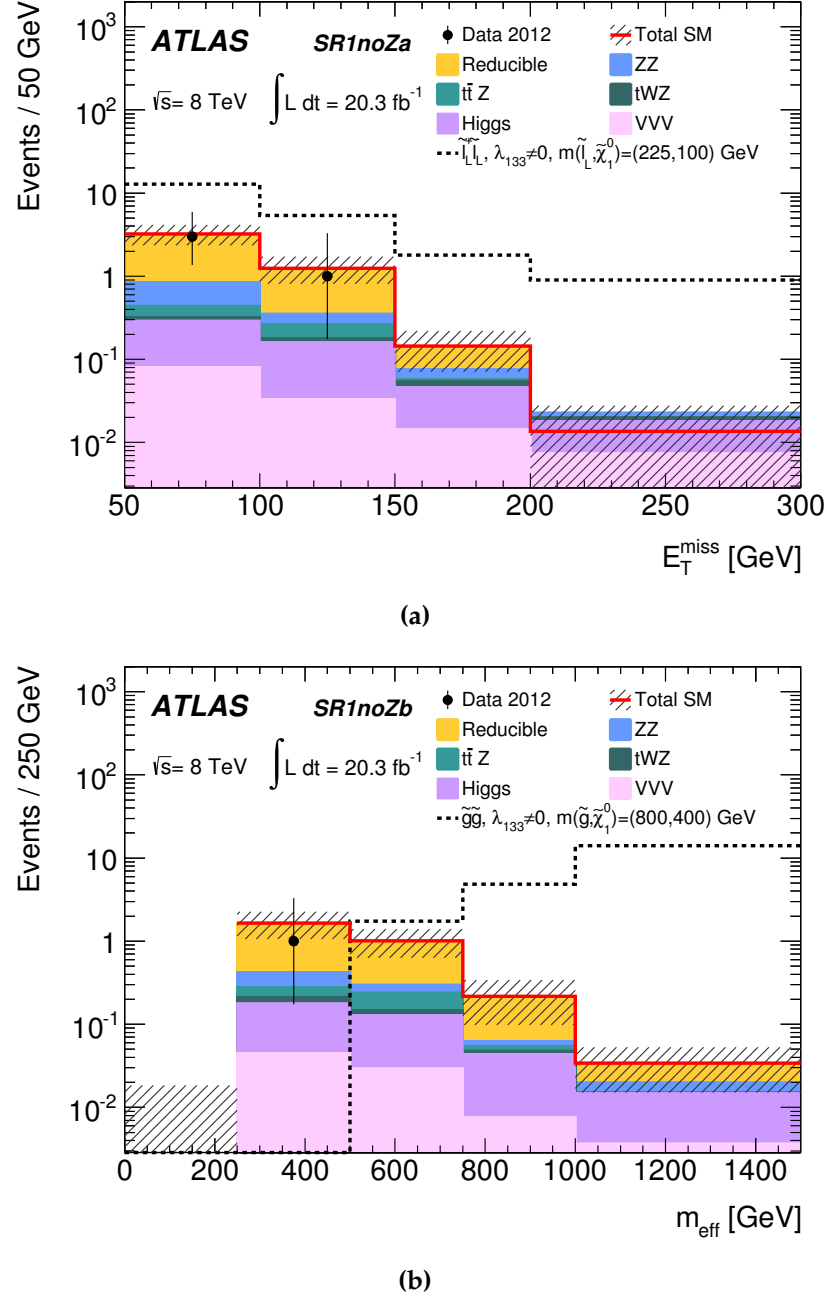
Figure 6.13: Predicted and observed distribution of the missing transverse energy in SR1noZa (a) and the effective mass in SR1noZb (b). The dashed line indicates an example signal from the simplified RPV model with an L-slepton NLSP and a \lambda_{133} LLE coupling (a) or the RPV simplified model with a gluino NLSP and a \lambda_{133} LLE coupling (b).
