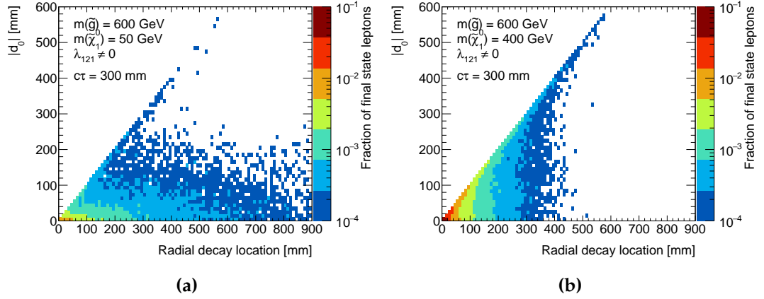
Figure 7.1: Transverse impact parameter |d_0| of final state leptons vs. the radial location of the neutralino decay vertex for the simplified RPV model with a gluino NLSP, c\tau = 300 mm, m_{\tilde{g}} = 600 GeV and a neutralino mass of m_{\tilde{\chi}_1^0} = 50 GeV (a) or m_{\tilde{\chi}_1^0} = 400 GeV (b).
