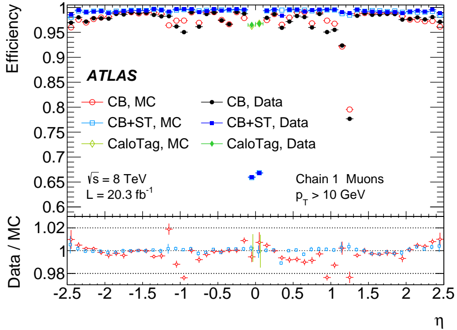
Figure 4.3: Muon reconstruction efficiency as a function of the pseudorapidity for combined muons (red/black) and the combination of combined and segment-tagged muons (blue). For the central pseudorapidity region, the efficiency of Calorimeter-tagged muons is shown in green.
