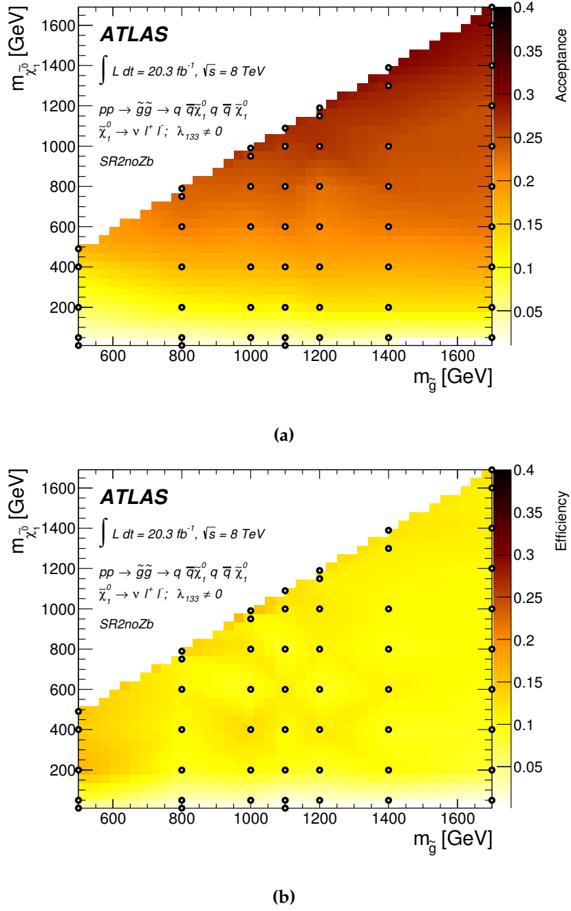
Figure 6.5: Acceptance (a) and efficiency (b) of the SR2noZb signal region for the simplified model with gluino NLSP and active \lambda_{133} coupling in the gluino-neutralino mass plane.
