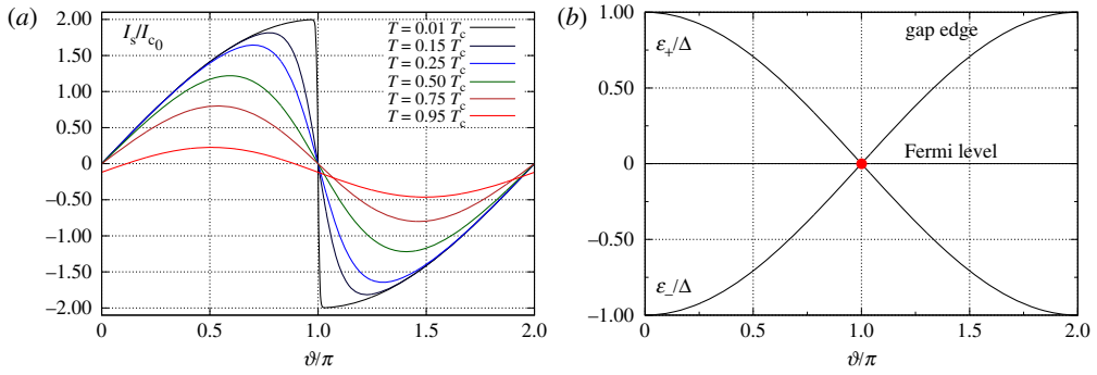
Figure 5. (a) Josephson current as a function of phase bias and temperature for a Sharvin point contact. The current is normalized in units of the Ambegaokar–Baratoff critical current at T = 0 , I_{c0} = \pi \Delta(0)/2e R_N . (b) Branches of Andreev bound states of a Sharvin point contact Josephson weak link dispersing as a function of the phase bias, \vartheta . (Online version in colour.)
