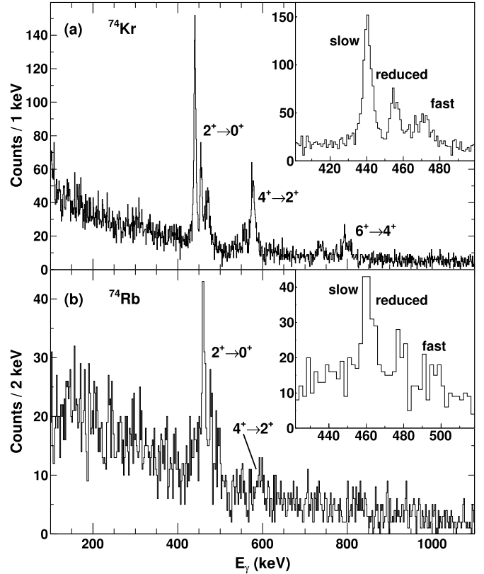
Fig. 2. Doppler-corrected \gamma -ray spectra detected in coincidence with (a) ^{74}\text{Kr} recoils and (b) ^{74}\text{Rb} recoils. For ^{74}\text{Kr} , several states are clearly populated, including the 2_1^+ , 4_1^+ , and 6_1^+ states. In contrast, only the 2_1^+ state is strongly populated in ^{74}\text{Rb} , with a small population of the 4_1^+ state visible. The insets show a closer view of the 2_1^+ \rightarrow 0_1^+ transition for each nucleus, with the fast, reduced, and slow components labeled. The data in both panels were taken with 1 mm separations between the target/first degrader and between the first degrader/second degrader, and the Doppler correction was performed using the velocity after the first degrader.
