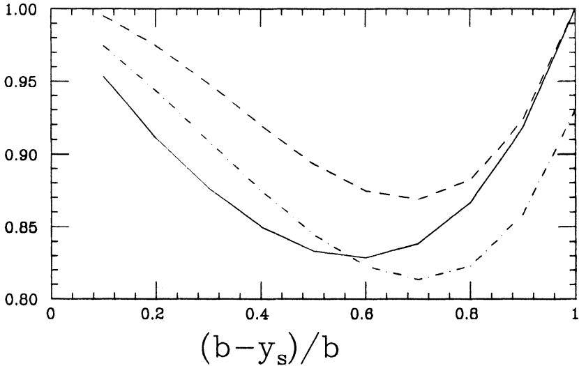
FIGURE 11: Loss parameter k_L for long bunch with fixed distance d=b-y_s between the beam and the wall. The horizontal axis is d divided by the half aperture b of the pipe. The loss parameter is normalized by that for the beam at the center of a round pipe with radius b=d .
