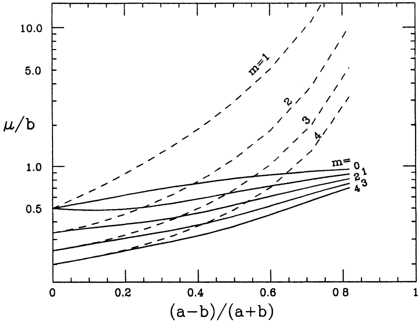
FIGURE 2: Eigenvalues (normalized by b ) for elliptic pipes as a function of (a-b)/(a+b) . The solid lines are cosine-like modes and the dashed lines sine-like.
