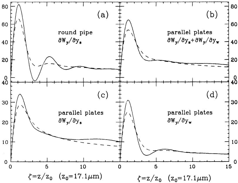
FIGURE 7: Transverse wake function with the AC conductivity taken into account for round pipe (a) and parallel plates (b,c,d) with b=1\text{cm} . (a) and (c) are \partial W_y / \partial y_s , (b) is \partial W_y / \partial y_s + \partial W_y / \partial y_w and (d) is \partial W_y / \partial y_w in units of 10^{12} V/C/m 2 . The dashed lines are those with DC conductivity.
