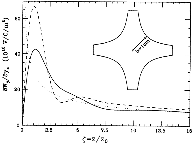
FIGURE 5: Transverse wake function (solid line) for a hyperbolic pipe with b=1\text{cm} . The dotted line is the asymptotic form and the dashed line is for the round pipe with radius 1\text{cm} .
