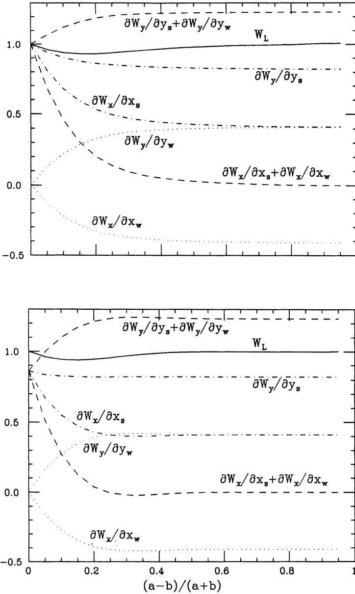
FIGURE 8: The coefficients of the asymptotic forms of the wake functions for elliptic pipes with the radii a and b (top) and for rectangular pipes with the width 2a and the height 2b (bottom) as functions of (a-b)/(a+b) . The values are normalized by those of the round pipe with radius b .
