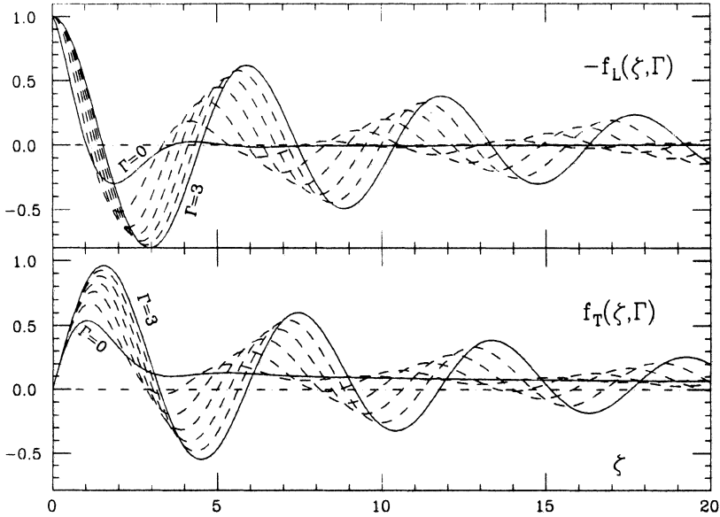
FIGURE 13: The functions f_L(\zeta, \Gamma) (top) and f_T(\zeta, \Gamma) (bottom) as functions of \zeta for \Gamma=0 and 3 (solid lines) and for the values in between with step 0.5 (dashed lines).
