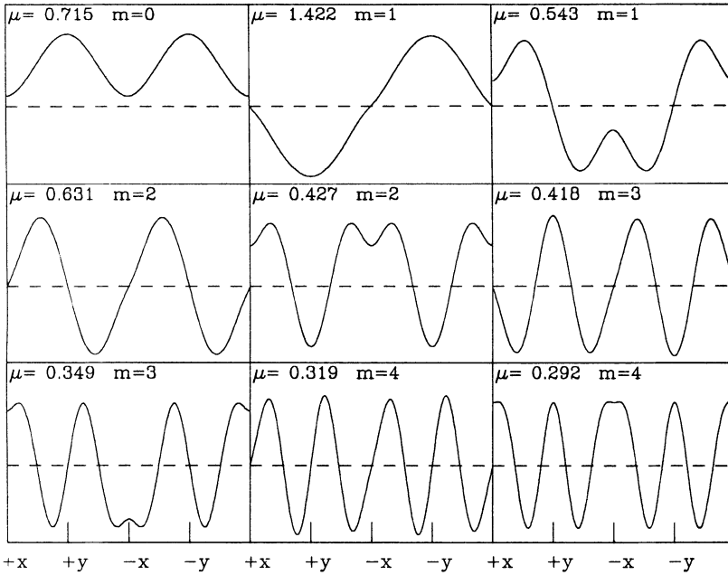
FIGURE 1: Eigenfunctions for an elliptic pipe with radius a/b=2 . The horizontal axis is the circumference of the cross section. The left edge corresponds to the positive x -axis and the first quarter point to the positive y -axis, etc., as indicated at the bottom. The eigenvalue (divided by b ) and the mode identification are indicated at the top of each graph.
