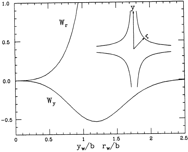
FIGURE 10: Transverse asymptotic wake for a hyperbolic pipe for r_w on the y -axis ( W_y ) and on the 45-degree line ( W_r ).
