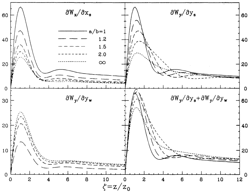
FIGURE 4: Transverse wake function for elliptic pipes with b=1\text{cm} .
