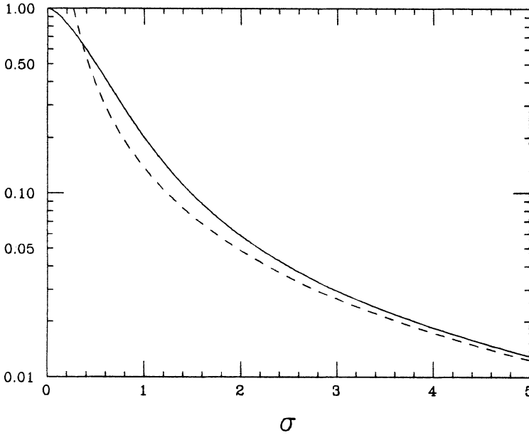
FIGURE 14: Function g_L(\sigma) (solid line) and its asymptotic form (dashed line) given in eq.(A.96).
