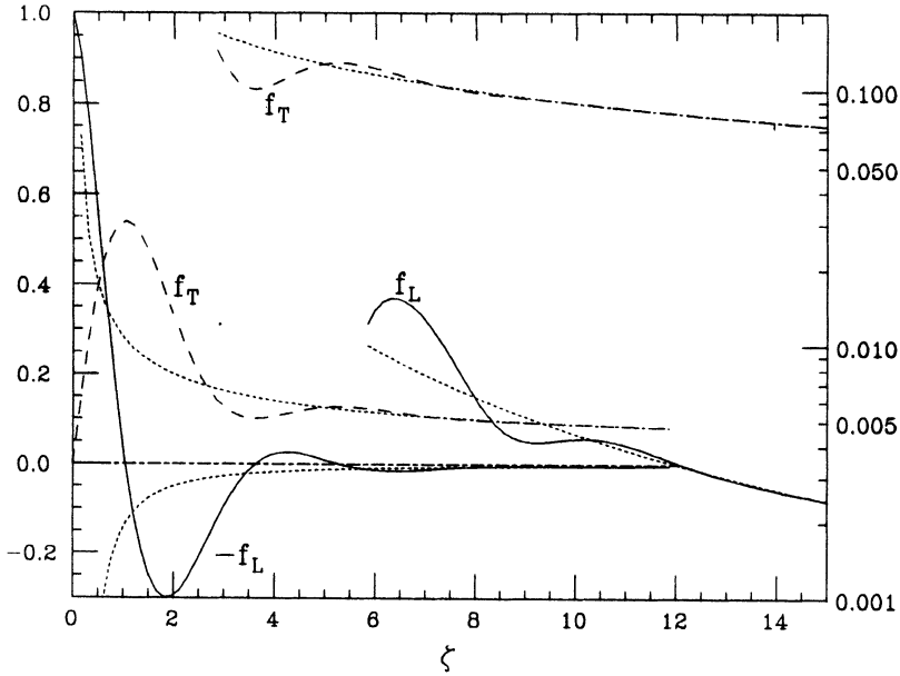
FIGURE 12: The basic wake functions f_L (solid) and f_T (dashed) and their asymptotic forms (dotted) defined in eqs.(A.82) and (A.83). The large \zeta region is plotted in logarithmic scale too (scale on the right).
