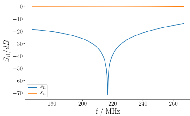
Figure 6: S-Parameters of the coupler after optimization.
