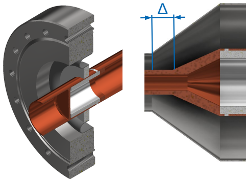
Figure 3: Window-Flange with ceramic window, u-shaped spring and connection jack with inner conductor mounted to one side (left side); conical adjustment of diameter transition from 3\frac{1}{8} to 14 mm rigid line (right side).
