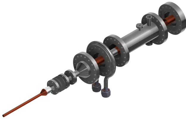
Figure 2: New modular design of the power coupler with two window-flanges.
