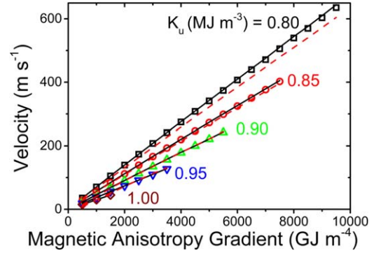
Figure 3. Dependence of skyrmion speed on magnetic anisotropy gradient for a range of magnetic anisotropy values at the centre of the skyrmion. The black solid line and the red broken line represents the analytical solution derived using the gradient force and bilayer coupling force respectively.
