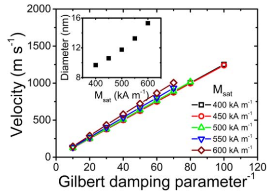
Figure 4. Dependence of skyrmion velocity on the inverse of Gilbert damping parameter and saturation magnetization. Inset shows the skyrmion diameter dependence on saturation magnetization.
