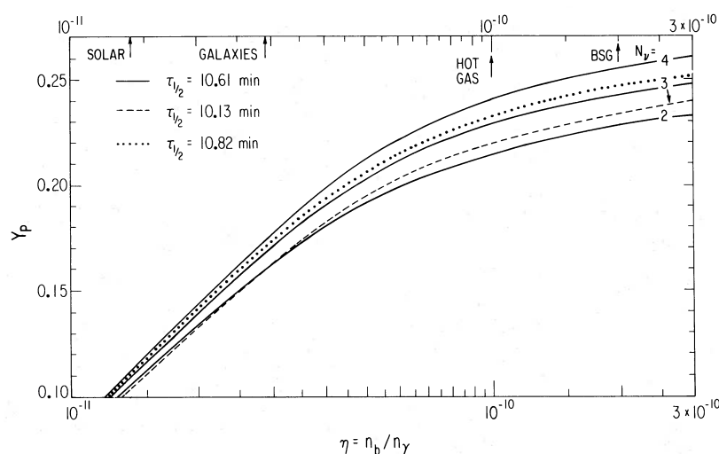
Figure 1. The helium mass fraction as a function of the baryon-to-photon ratio for three choices of N_\nu = 2, 3, and 4 and three choices of \tau_{1/2} with N_\nu = 3 . Figure circa 1981 from ref. [13].
