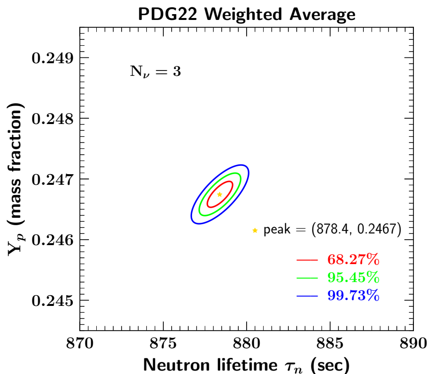
Figure 6. The sensitivity of the ^4\text{He} abundance to the neutron mean lifetime, assuming a Gaussian distribution for \tau_n with mean and uncertainty given by Equation (2). In addition to the peak of the likelihood, denoted by a star, we show the 1, 2, and 3\sigma contours.
