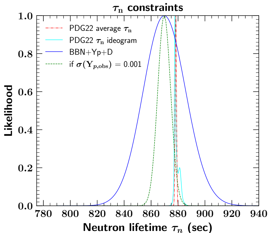
Figure 10. Comparison of the current and potential future BBN predicted likelihood function for \tau_n with the experimental likelihood. The solid blue curve shows the current BBN prediction, which is tightened to the green dashed curve if the uncertainty in the helium mass fraction can be reduced to \sigma_{\text{obs}}(Y_p) = 0.001 . For comparison, the red dot-dashed curve shows the experimental value for \tau_n represented by a Gaussian. The distribution represented by the ideogram is shown by the thin cyan solid curve.
