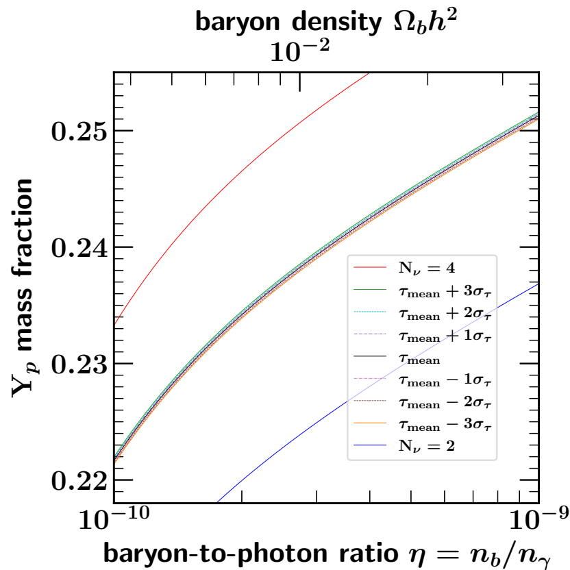
Figure 5. The helium mass fraction as a function of the baryon-to-photon ratio for three choices of N_\nu = 2, 3 , and 4 and for a spread in values of \tau_{1/2} up to \pm 3\sigma about the mean with N_\nu = 3 .
