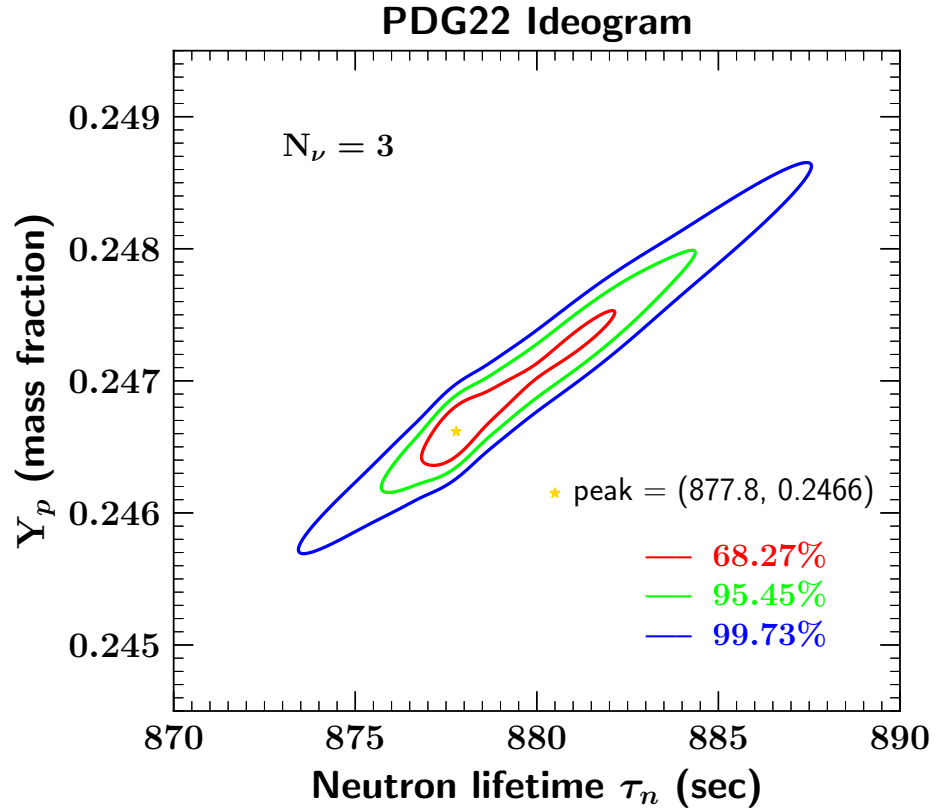
Figure 7. As in Figure 6 where we have assumed the distribution of \tau_n taken from the ideogram in Figure 3b.
