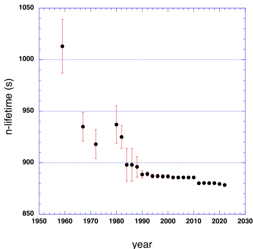
Figure 2. The average mean lifetime of the neutron as compiled by the Review of Particle Properties/Physics. Please note that the uncertainty in the mean life for more recent measurements is smaller than the symbol showing the mean.
