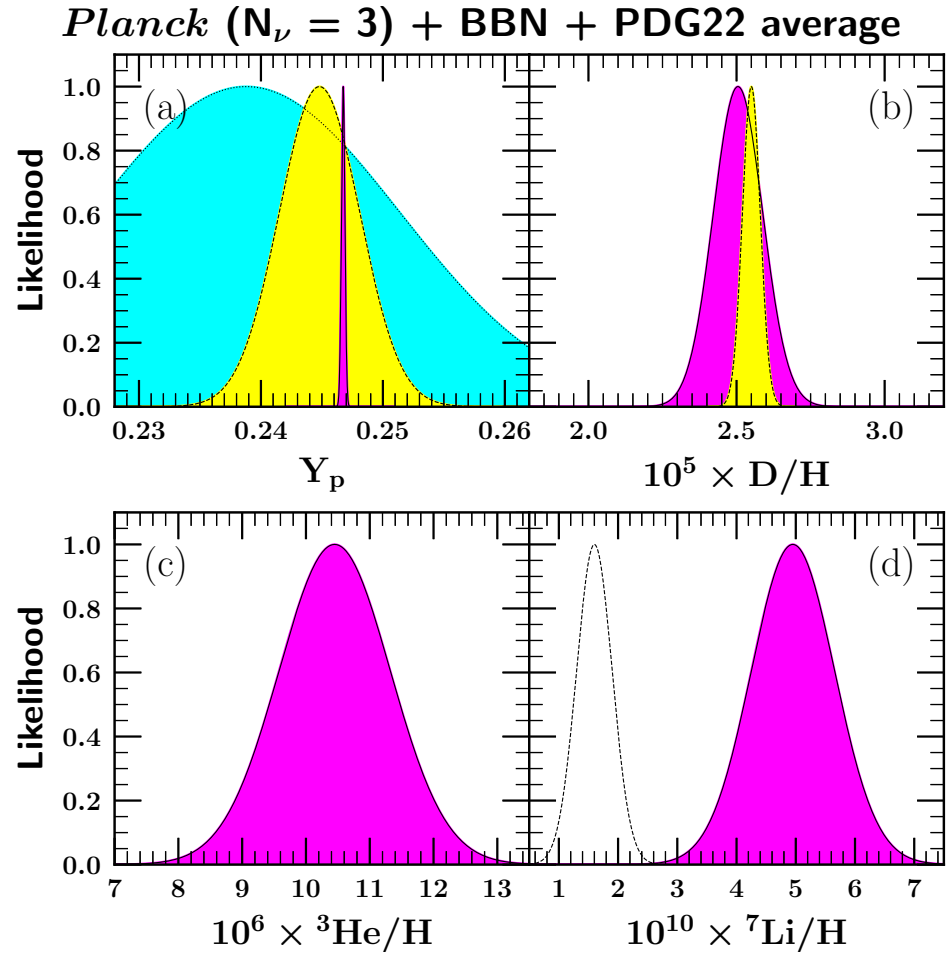
Figure 8. Light element abundance likelihood functions. Shown are the likelihoods for each of the light nuclides: (a) the ^4\text{He} mass fraction, Y_p , (b) \text{D}/\text{H} , (c) ^3\text{He}/\text{H} , and (d) ^7\text{Li} . The solid-lined, dark-shaded (purple) curves are the BBN+CMB predictions, based on Planck inputs as discussed in the text. The dashed-lined, light-shaded (yellow) curves show astronomical measurements of the primordial abundances, for all but ^3\text{He} where reliable primordial abundance measures do not exist. For ^4\text{He} , the dotted-lined, medium-shaded (cyan) curve shows the independent CMB determination of ^4\text{He} .
