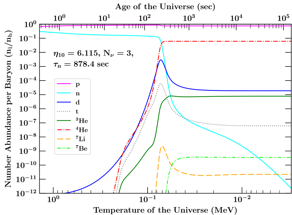
Figure 4. Time evolution of the light element abundances during BBN. Please note that time (upper axis) increases to the right, and so the temperature is shown to decrease to the right.
