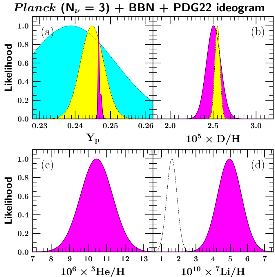
Figure 9. As in Figure 8, where the neutron mean life is selected from the ideogram in Figure 3b rather than the Gaussian distribution.
