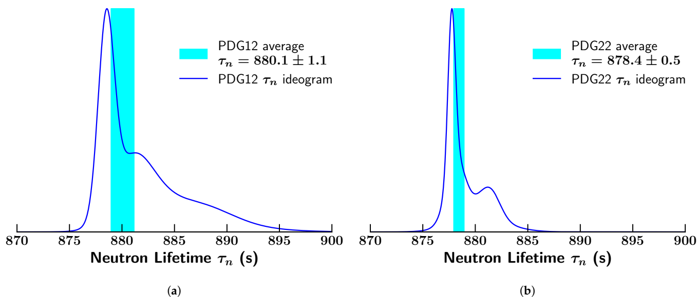
Figure 3. Ideograms for neutron lifetime measurements. (a) Ideogram for the seven measurements contributing to the PDG average neutron mean life in 2012; (b) Ideogram for the eight measurements contributing to the PDG average neutron mean life in 2022.
