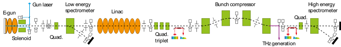
Figure 1: Schematic overview of the FLUTE layout showing the diagnostics and magnets [10].
