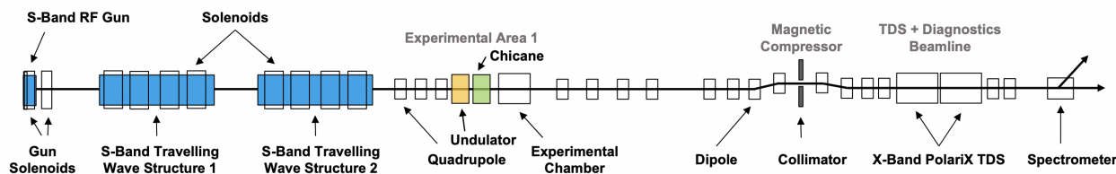
Figure 2: Schematic overview of the ARES layout.
