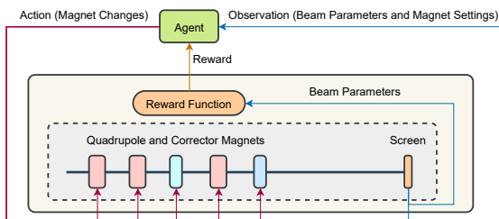
Figure 3: RL environment for beam optimisation in the ARES EA. The RL environment is shown in beige with the accelerator (or simulation) shown in grey. Quadrupoles are denoted in red, cyan and blue denote vertical and horizontal correctors respectively.
