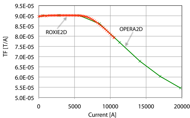
Figure 3: Transfer function of the quadrupole magnet. (Reference radius: 40 mm)
