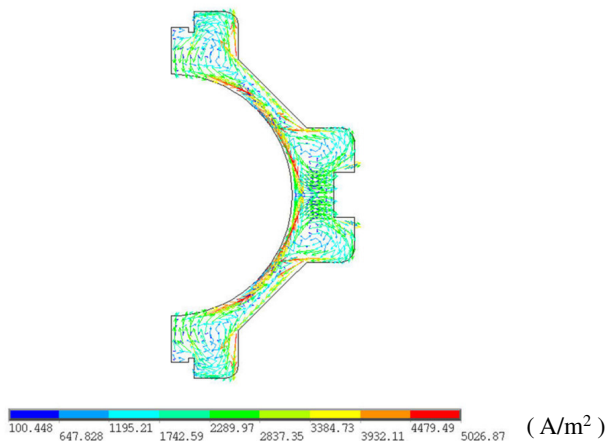
Figure 8: FEM model of the connection flange (half) of the quadrupole magnet.
