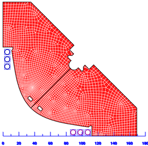
Figure 2: Cross section of the SIS100 main quadrupole magnet (quadrant) and the reference radius (40 mm).
