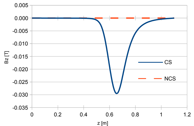
Figure 5: Magnetic field along beam axis ( B_z ) at the magnet aperture center at the connection side (CS) and non connection side (NCS). I = 7.3 kA.
