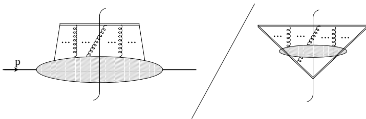
Fig. 3. Diagrammatic interpretation of Eq. (18). This is ordinary pdf in coordinate space (with a light-like Wilson line) divided by the vacuum expectation value of a certain pure Wilson line operator. Any number of gluon lines can join the lower blob to the top Wilson line in the numerator. Any number of gluon lines can join the Wilson lines in the denominator.
